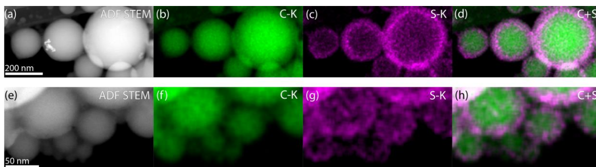
Figure 6. STEM-EDX K-edge maps demonstrating the smallest feature size that can be measured. (a-d) Mapping of 1:1 TQ1:PC 71 BM nanoparticles of diameter 150 to 350 nm, and (e-h) of diameter 30 to 100 nm. In order (a, e) HAADF, (b, f) C (green), (c, g) S (purple), (d, h) overlay of C (green) and S (purple).
