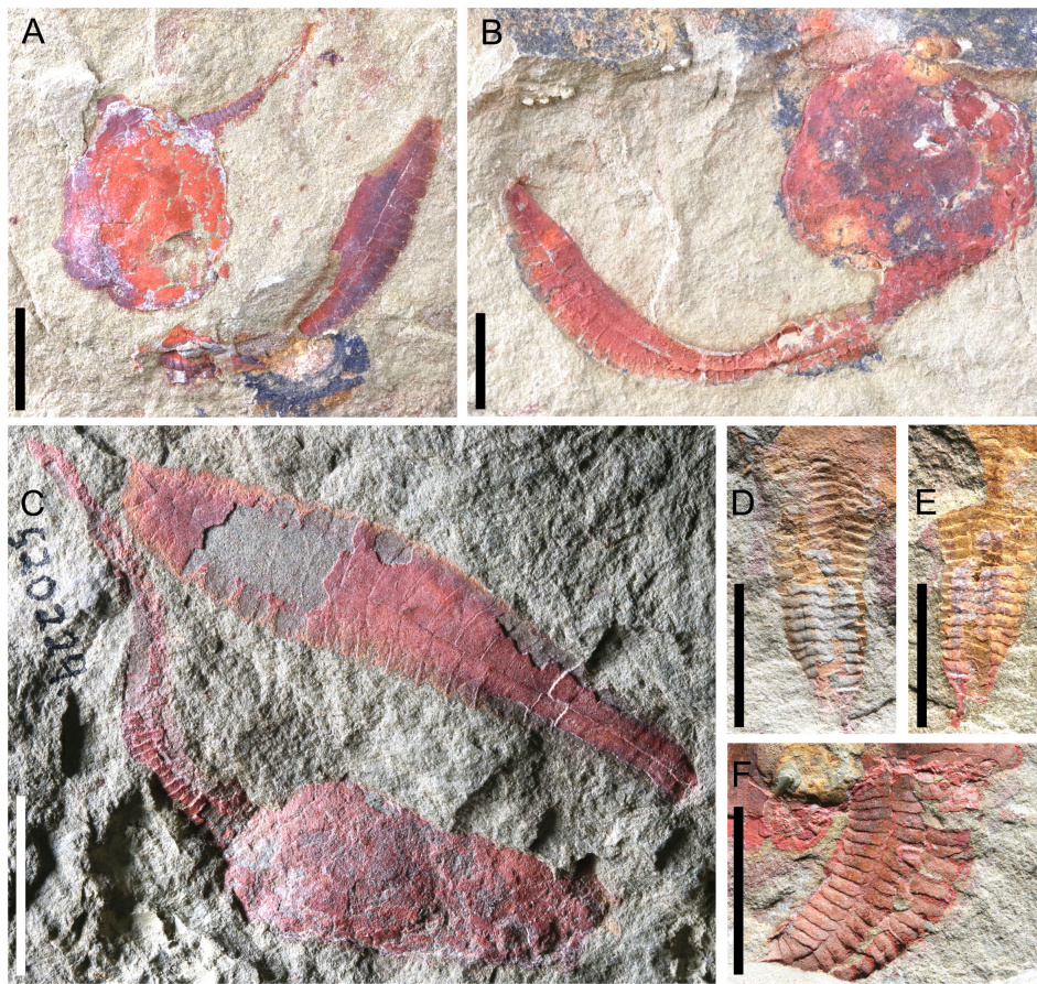
FIGURE 10 Photographs of Nimchacystis agterbosi from the Z-F17b locality (late Tremadocian). (A) Holotype UCBL-FSL.713120 showing theca, feeding appendage, proxistele, and dististele in near anatomical connectivity as in life. (B) SMF.89671 showing theca and stele in anatomical connection. (C) YPM.IP.520029 showing a large specimen with an apparently complete feeding appendage and dististele. (D) YPM.IP.520031 part showing a complete and well-preserved proxistele. (E) YPM.IP.520031 counterpart showing a complete and well-preserved proxistele. (F) YPM.IP.520370 showing a complete and well-preserved proxistele. Scale bars = 10 mm. Photographs (A) and (B) by Vincent Perrier. Photographs (C) to (F) by Jessica Utrup
