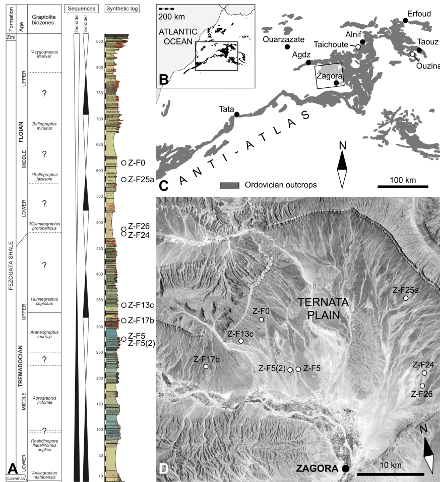
FIGURE 1 Stratigraphic and geographic occurrences of solutan echinoderms in the Fezouata Shale (Lower Ordovician), Anti-Atlas, Morocco. (A) Stratigraphic position of solutan localities in the Ternata plain (Zagora area, Central Anti-Atlas). Graptolite biozonation, eustatic sequences, and synthetic log (left columns) are based on Lefebvre et al. (2016); Lefebvre et al. (2018). Colours on the log correspond to those of the rocks on the outcrop. (B) Simplified geological map of northwestern Africa showing the distribution of Ordovician rocks and the location of the Anti-Atlas. (C) Simplified geological map of the Anti-Atlas showing the distribution of Ordovician rocks and the location of the three main areas yielding Early Ordovician solutan remains: Ternata plain (Zagora area), western Maider (Taichoute), and Taouz Massif (Ouzina). (D) Landsat view of the Ternata plain (Zagora area, Central Anti-Atlas) showing the location of all main Early Ordovician solutan localities mentioned in the text and specified on the log; photograph courtesy of the U.S. Geological Survey.
