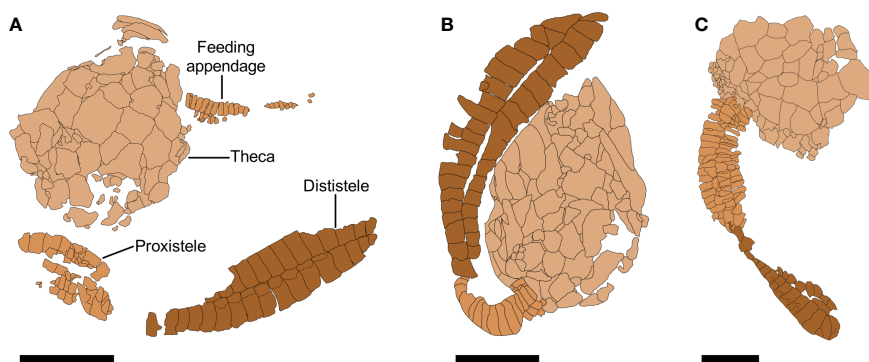
FIGURE 11 Camera lucida drawings of Nimchacystis agterbosi . (A) Holotype UCBL-FSL.713120 showing theca, feeding appendage, proxistele, and dististele almost in near anatomical connectivity as in life. (B) UCBL-FSL.713058 showing an almost complete dististele. (C) SMF.89671 showing theca and stele in anatomical connection. Scale bars = 10 mm.
