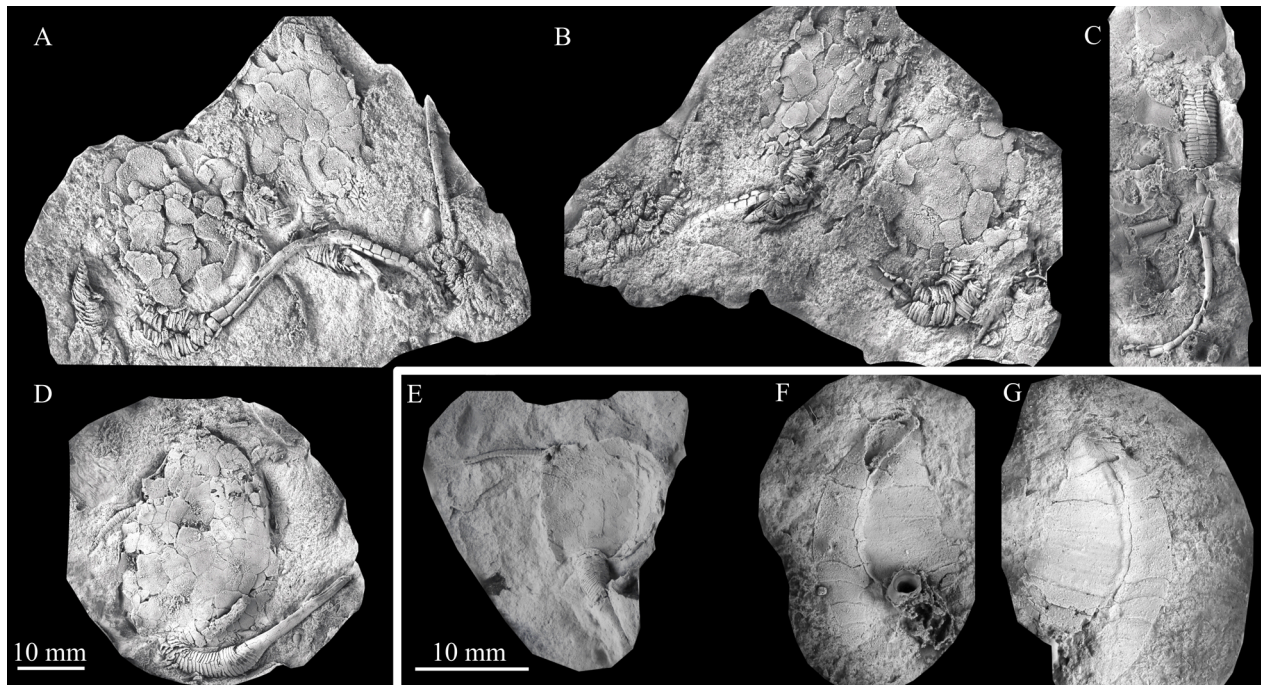
Fig. 1. Solutans from the Saint-Chinian Formation (upper Tremadocian), Montagne Noire (Hérault, France); latex casts of original specimens; A–E , Minervaeocystis vidali (Thoral, 1935); A–B , cluster of four individuals (part and counterpart), BMNHUK.E.23695 (Miquel coll.), Cassagnoles; A , nearly complete individual (in lower aspect) in the centre of the cluster, with fully articulated brachiole and long, strongly curved, twisted dististele; B , same individuals (in upper aspect); C , well-preserved individual (in lower aspect) with strongly curved, twisted dististele; UCBL.FSL.713595 (Kundura coll.), Prades-sur-Vernazobre; D , fully articulated theca (in upper aspect) with brachiole and well-preserved anal pyramid, right of homoiostele insertion; lectotype, UM.AC1.634 (Villebrun coll.), Saint-Chinian; E , juvenile individual, UM.AC1.636 (Thoral coll.), Prades-sur-Vernazobre; F–G , Plasiacystis mobilis Prokop & Petr, 2003; latex casts of the dististele (part and counterpart) of the single known specimen (MBB.GG.6, Griffé coll.), Saint-Chinian; note the presence of a well-defined spike-shaped tubercle on one of the two sides ( F ).
