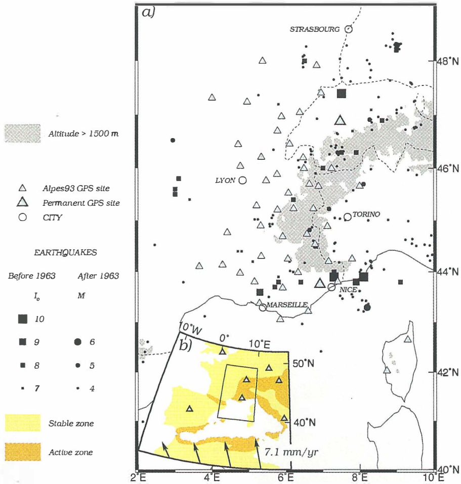
Fig. 1. a) The area covered by the GPS network in the Western Alps. Earthquakes before 1963 are indicated by dark squares; earthquakes that struck after 1963 are depicted by dark circles. Triangles indicate GPS sites as detailed in the legend. b) The inset at the lower left of the figure shows the tectonic framework of the Western Mediterranean region. Black arrows indicate the motion of the African plate relative to the Eurasian plate (Courtesy of Charles DeMets).
