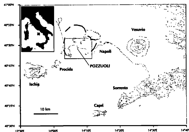
Figure 1. Location of the investigated area: topography of the region of Napoli and Mt. Vesuvio (200-m contour lines). Inset selection corresponds to the Campi Flegrei area used for modelling (Pozzuoli Bay). The black thick line represents the inland caldera rim.
