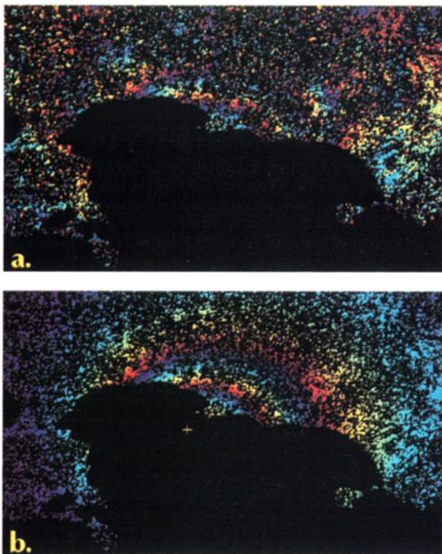
Figure 4. Modelling of the deflation by a source point in elastic half-space ( 11.6 \times 9.4 km area). (a) Data used for the inverse problem (selection of most coherent pixels in the interferogram). (b) Best model found: computed interferogram and location of the 2.7-km deep source (cross).
