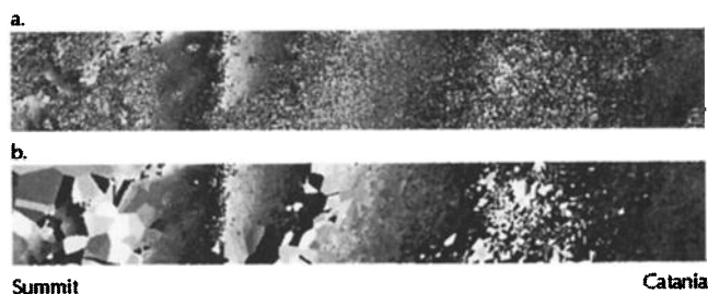
Figure 6. Example of interpolation by the nearest neighbor method on the selected area (1200 × 100 pixels) from Catania to summit (interferogram 54). (a) Original phase values. (b) Interpolated data after the applying of collective mask. Note the unsmoothed phase wrapping (transitions black to white) that are kept intact and will favor phase unwrapping.
