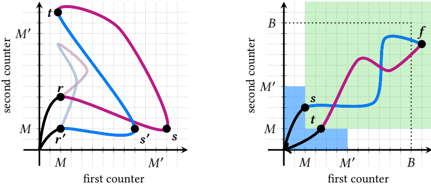
Fig. 14. Illustrations of the proof of Theorem 5.1. Left : we identify two path segments, one from r to t via s (in \blacksquare ), and one from t to r' via s' (in \blacksquare ). Both can be shortened via Lemma 5.15 (applied to the reverse of the second segment). Composing the shortenings produces a new path from 0 to 0 , in which the point corresponding to t has moved vertically down. Right : shortest paths cannot leave the shaded area. The path from s to t via a sufficiently large point f can be shortened using Lemma 5.16.
