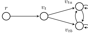
Fig. 9. An abstract graph for the RPN in Figure 1
