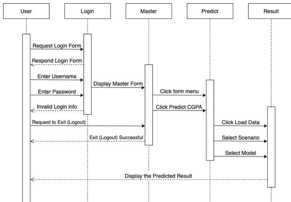
Figure 2. System Sequence Diagram
