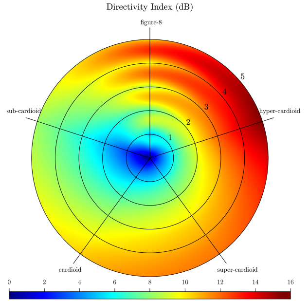
Fig. 6: Directivity Index (in dB). Up to order N = 5 .
