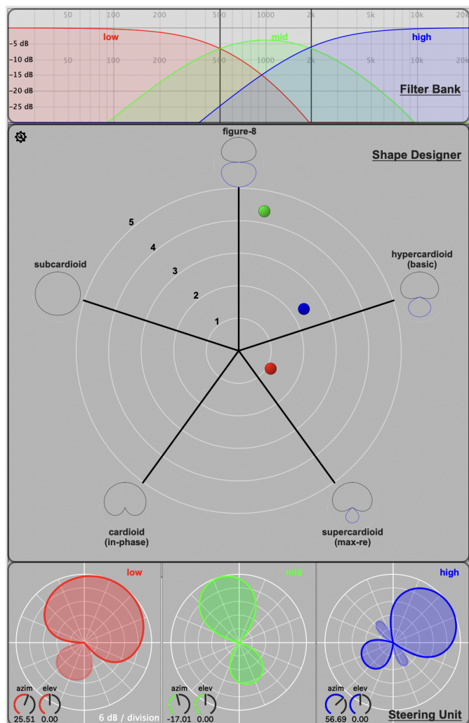
Fig. 9: GUI for the radiation shape designer (here presented for N = 5 ). (a) Top: 3-band filter bank. (b) Middle: directivity shape designer. (c) Bottom: directivity steering unit.
