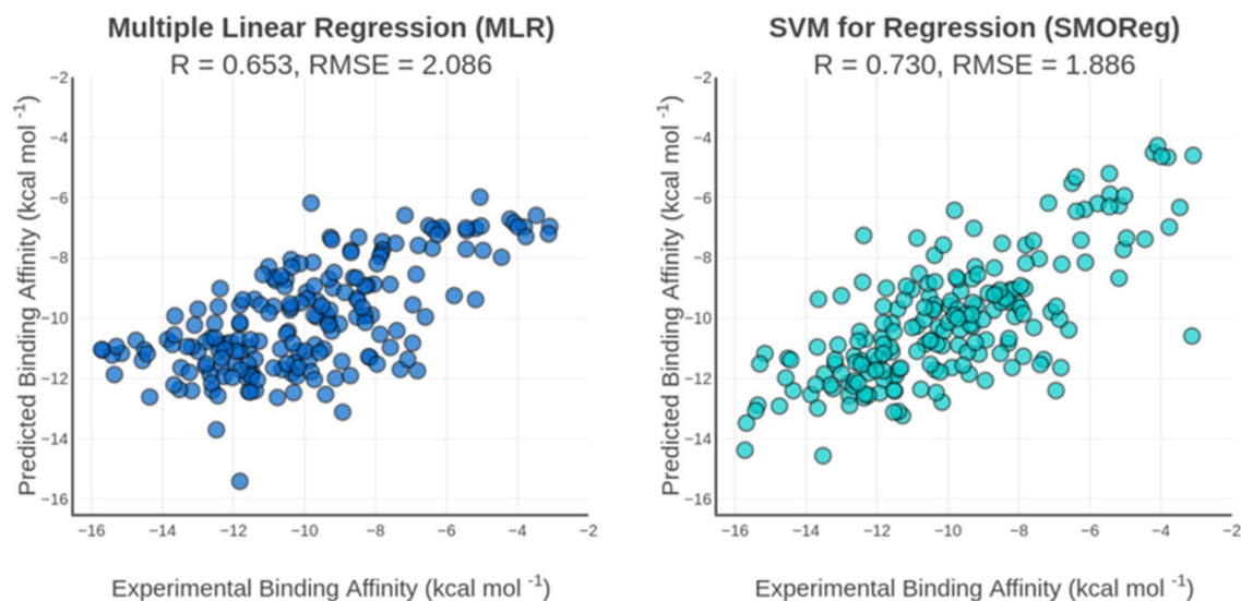
Figure 3. Correlation plot of experimental and predicted binding affinities by MLR (left) and SMOReg (right) specific scoring functions for proteases. The scoring functions were evaluated on the independent test set for proteases ( N = 196 ). R is the Pearson's correlation coefficient and RMSE is the root mean squared error given in \text{kcal mol}^{-1} .
