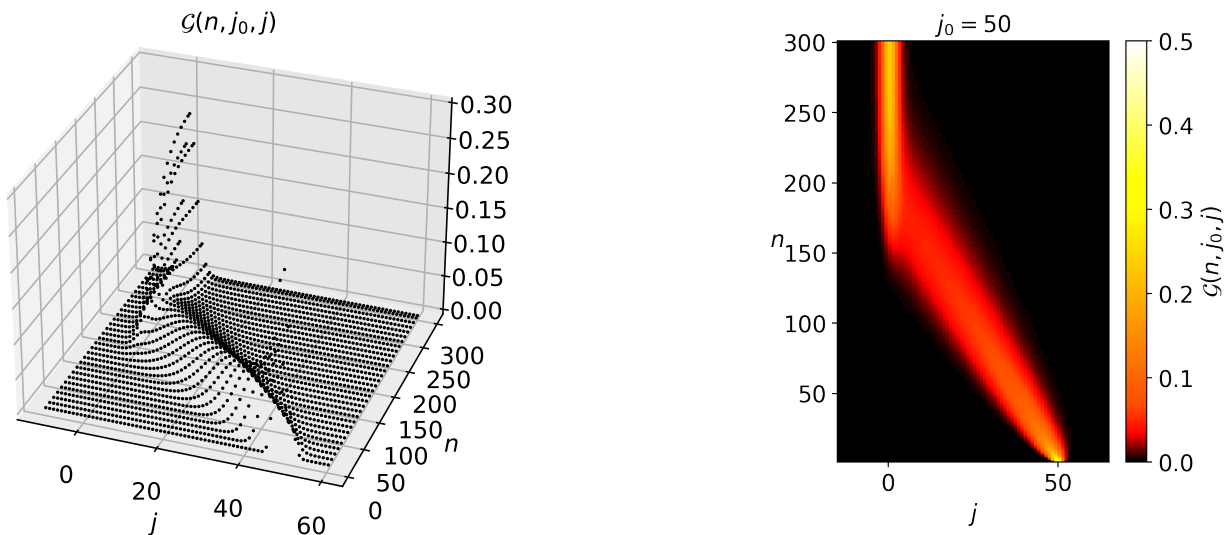
Figure 5: Representation of the Green's function \mathcal{G}(n, j_0, j) for j_0 = 50 . The initial time n = 0 has been removed for readability since the Green's function is equal to the sequence \delta_{j_0} at this time step.
