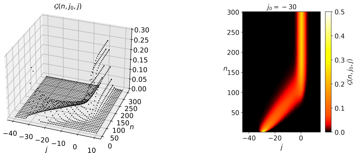
Figure 6: Representation of the Green's function \mathcal{G}(n, j_0, j) for j_0 = -30 . The initial time n = 0 has been removed for readability purposes since the Green's function is equal to the sequence \delta_{j_0} at this time step.
