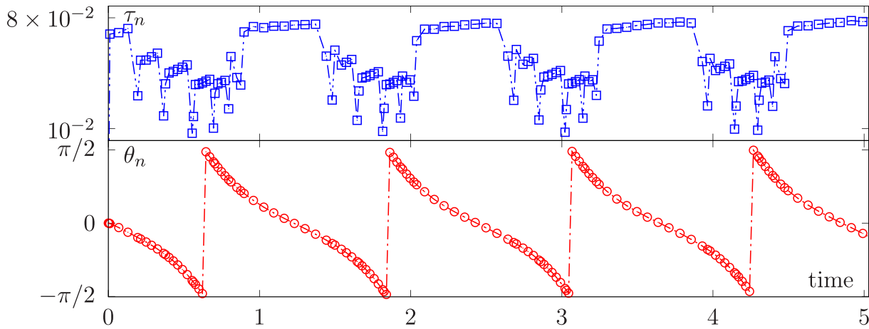
FIGURE 14 Example 3: Adapted time-step size \delta t_n and corresponding inclination angle \theta_n when the fully periodic TB regime is established. Parameters of the simulation: Re = 10^{-2} , Bn = 10^3 , and viscosity ratio is \beta = 10 . [Colour figure can be viewed at wileyonlinelibrary.com ]
