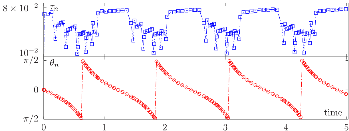
FIGURE 14 Example 3: Adapted time-step size \delta t_n and corresponding inclination angle and \theta_n when the fully periodic TB regime is established. Parameters of the simulation: Re = 10^{-2} , Bn = 10^3 , and viscosity ratio is \beta = 10 . [Colour figure can be viewed at wileyonlinelibrary.com ]
