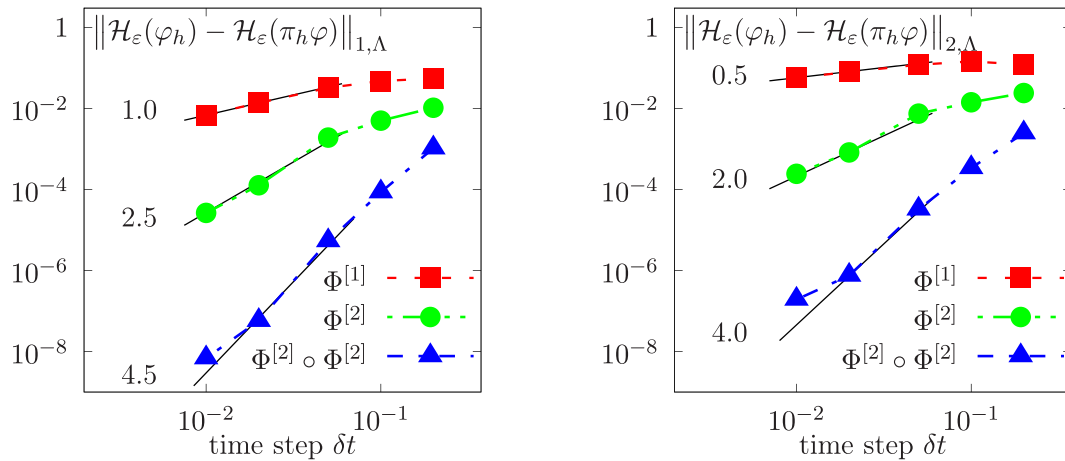
FIGURE 8 Example 2: Comparative study of the convergence rates in time for various numerical schemes. The errors are computed in the L^\kappa(\Lambda) norms with \kappa = 1, 2 . [Colour figure can be viewed at wileyonlinelibrary.com]
