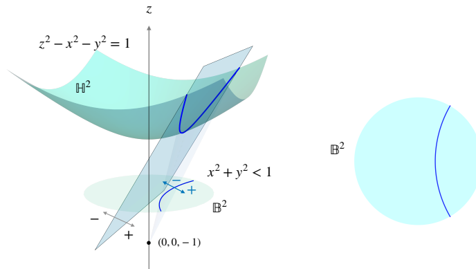
Figure 2: A geodesic in the hyperboloid model of the hyperbolic plane \mathbb{H}^2 , obtained as the intersection of a plane with the hyperboloid. The corresponding geodesic on the Poincaré disc model \mathbb{B}^2 of the hyperbolic plane is obtained by stereographic projection from the point (0, 0, -1) .
