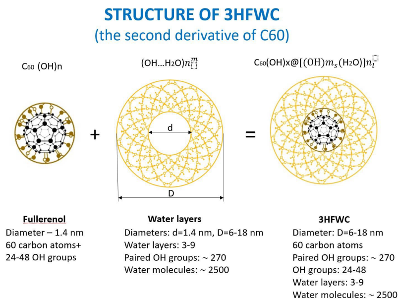
Figure 2: Structure, generated for 3HFWC by ACD/ChemSketch
