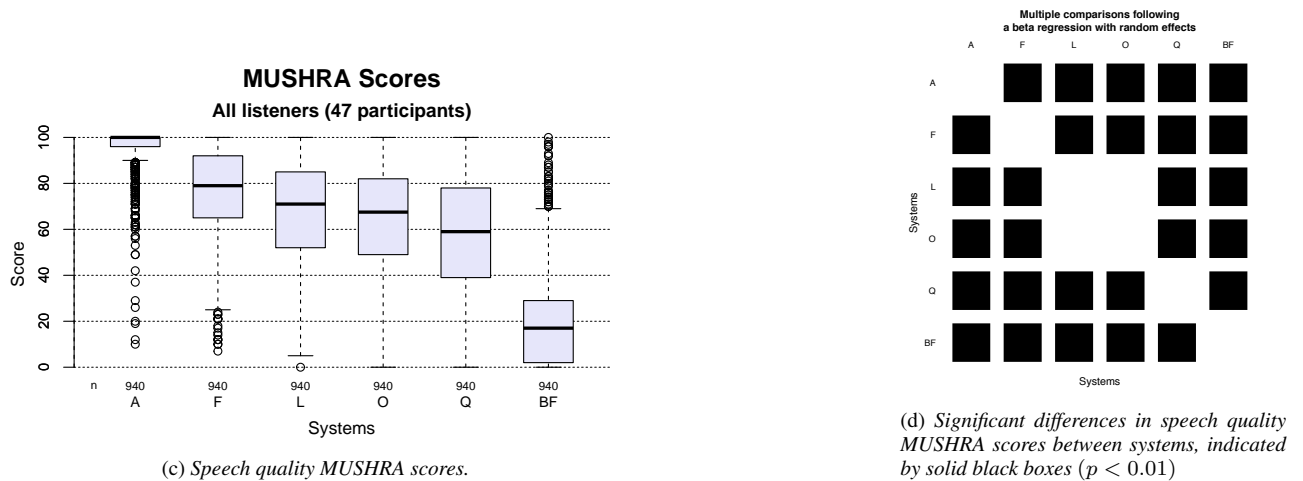
Figure 2: Speech quality results for FS1, with MOS (Test 4.a) and MUSHRA (Test 5) evaluations, per system.
