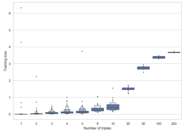
Figure 3: Final training loss of each experiment in the basic setup.
