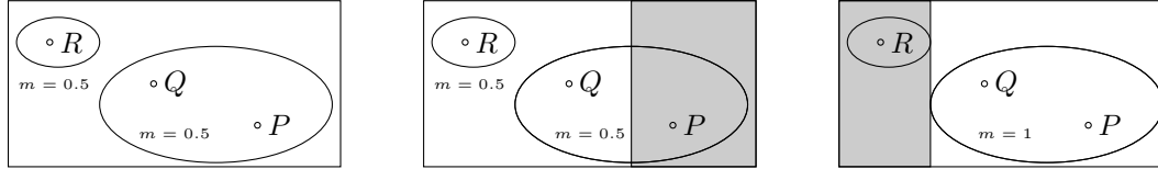
■ Figure 1 Prior (left) and posteriors given \{Q, R\} (center) and given \{P, Q\} (right). White and gray areas denote possible and impossible events – circles denote focal elements.
