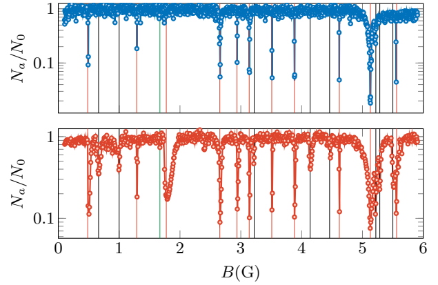
FIG. 1. Normalized atom number as a function of magnetic field for a thermal sample with temperature T = 190\text{ nK} (top panel in blue) and T = 2.4\text{ }\mu\text{K} (bottom panel in red). The red vertical lines indicate the 11 loss features for which we characterize the density and temperature dependence.
