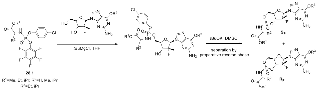
Scheme (28). Synthetic pathway to cyclic phosphoramidate prodrugs of 6-O-alkyl-2'-fluoro-2'-C-methyl guanosine. 28.2 , R 1 =Et, R 2 =Me, R 3 =Et
