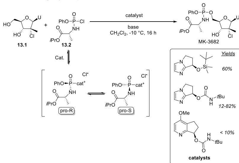
Scheme (13). Diastereoselective coupling via dynamic kinetic resolution.
