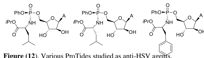
Figure (12). Various ProTides studied as anti-HSV agents.
