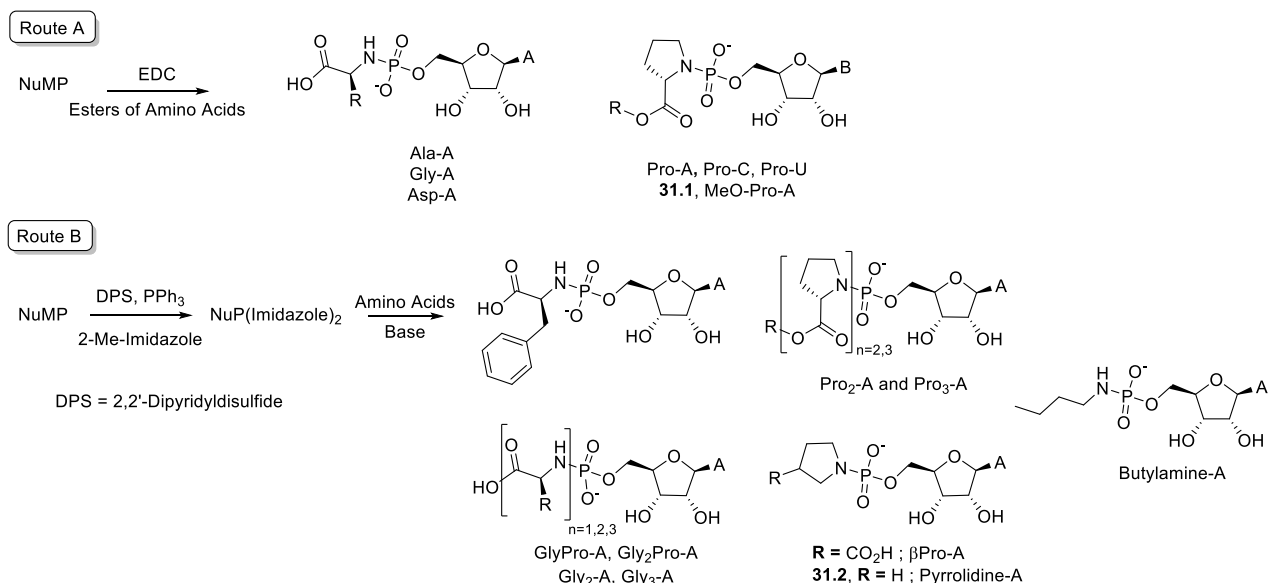
Scheme (31). Synthetic pathways to nucleoside 5'-phosphoramidate monoesters containing various amino-acids, di- or tripeptides, pyrrolidine or n-butylamine.
