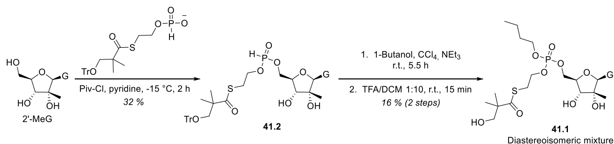
Scheme (41). Synthesis of the SATE phosphotriester derivative of 2'-C-methyl- \beta -D-guanosine.
