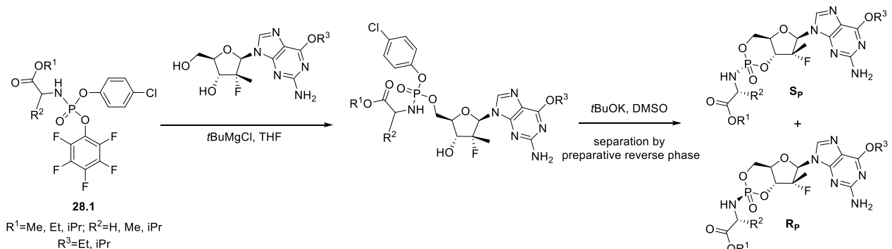
Scheme (28). Synthetic pathway to cyclic phosphoramidate prodrugs of 6-O-alkyl-2'-fluoro-2'-C-methyl guanosine. 28.2 , R 1 =Me, Et, iPr, R 2 =Me, R 3 =Et
