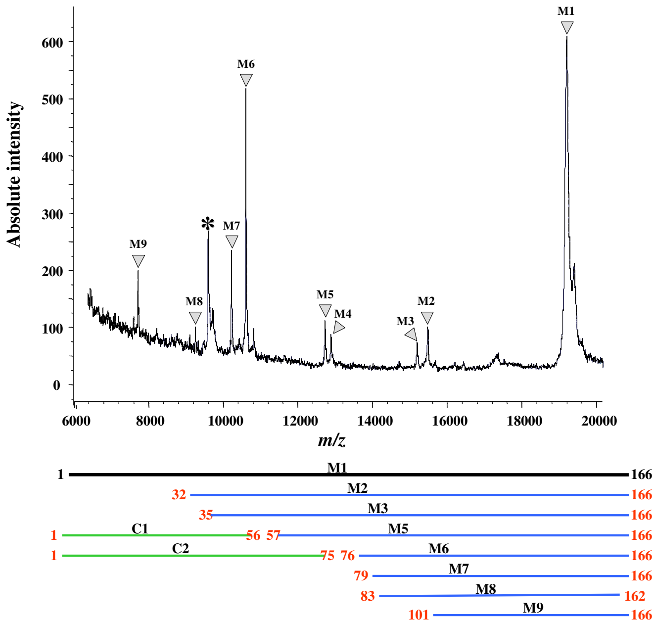
Figure 4 MALDI-TOF mass spectrum of large peptide fragments produced by SSO055 I partial trypsin proteolysis. A partial enzymatic proteolysis was carried out during 60 sec at 20°C with a trypsin/SSO055 I protein ratio of 1/20 (w/w). The products were then resolved onto a C8 reverse phase chromatographic column and the different UV absorbing fractions were analyzed by MALDI-TOF. The m/z spectrum obtained with the fraction eluting at 40–50 % acetonitrile is shown. The asterisk labels a peak arising from trypsin autolysis. Peaks that could be assigned are identified with numbers (experimental m/z , residues, Δmass in ppm compared to theoretical [M+H] + average mass): M1 (19198.4, [1–166], -1), M2 (15478.7, [32–166], -53), M3 (15191.2, [35–166], +153), M4 (12883.4, [52–162] or [56–166], -46 or -43), M5 (12724.2, [57–166], +193), M6 (10603.8, [76–166], +51), M7 (10220.1, [79–166], +77), M8 (9257.2, [83–162], +63) and M9 (7717.0, [101–166], -134). Peptides C1 and C2 , complementary of M5 and M6 , were not observed in this spectrum but in another fraction from the C8 reverse-phase chromatography corresponding to smaller peptides.
