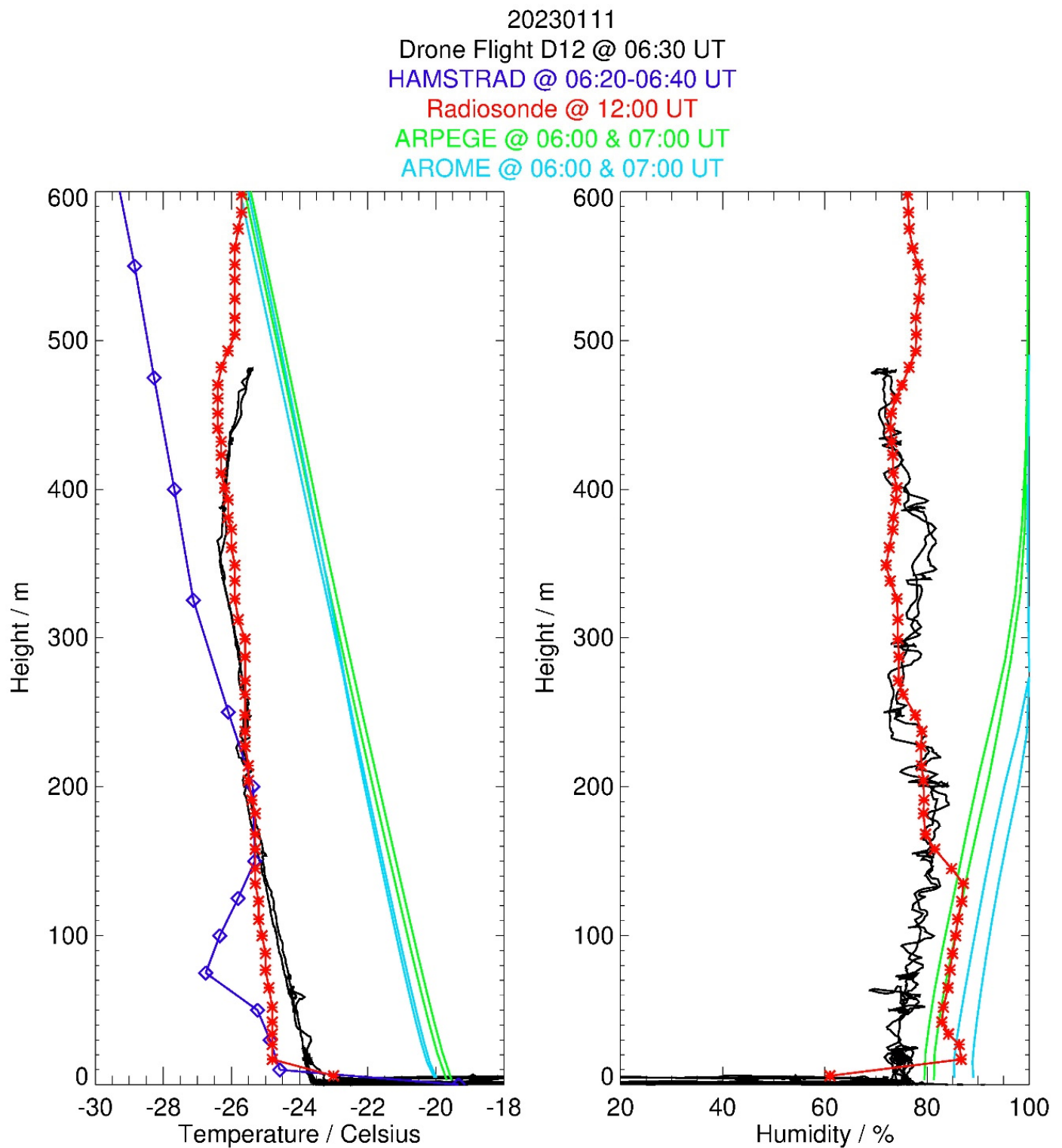
Figure 10. Same as Figure 6 but for flight D12 on 11 January 2023 at 06:30 UTC (black) and as observed by the balloon-borne sonde at 12:00 UTC (red). The HAMSTRAD temperature profile within 06:20–06:40 UTC is also shown in purple (left). The ARPEGE and AROME profiles calculated at 06:00 and 07:00 UTC are displayed in green and blue, respectively.
