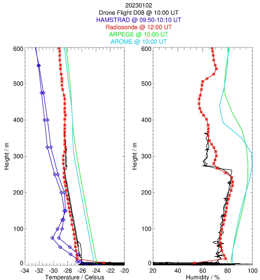
Figure 6. Vertical profiles of temperature ( left , ^{\circ}\text{C} ) and relative humidity ( right , %) measured by the Vaisala sonde onboard the drone during the ascending and descending flight phases for the flight D08 on 2 January 2023 around 10:00 UTC (black) and as observed by the balloon-borne sonde at 12:00 UTC (red). The HAMSTRAD temperature measurements within 09:50–10:10 UTC are also shown in purple ( left ). The ARPEGE and AROME profiles calculated at 10:00 UTC are displayed in green and blue, respectively.
