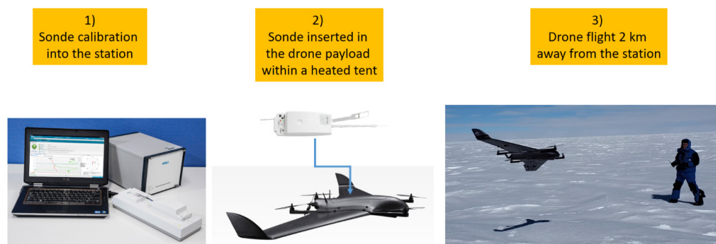
Figure 3. The methodology used for the scientific flights is synthesized as follows. (1) The Vaisala PTU sondes are calibrated into the quiet building of the Concordia station at room temperature using the standard Digicora system. (2) The PTU sonde is then transported to a heated tent about 500 m away from the station where the drone is stored. Then, the sonde is installed inside the drone. (3) The drone is transported with a skidoo to about 2 km away from the heated tent in the northward direction. There, it is launched following a previously validated flight plan.
