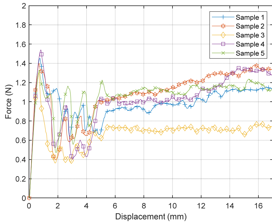
Figure 9. Debonding force measurement of the scotch tape.
