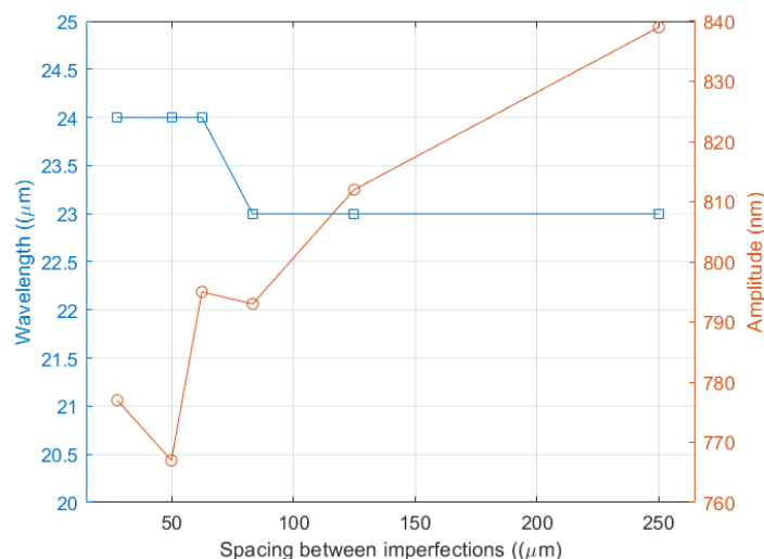
Figure 3. Wrinkling wavelength and amplitude vs. spacing between imperfections.
