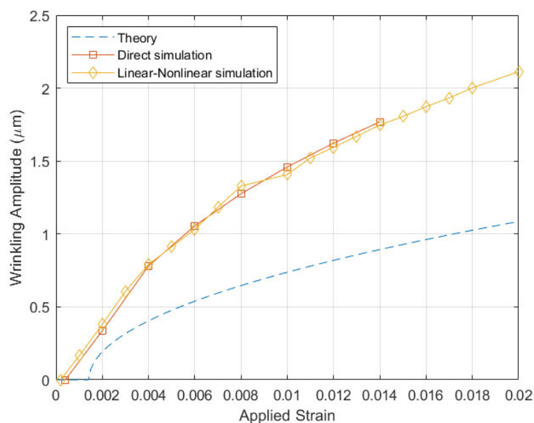
Figure 7. Wrinkling amplitude as a function of applied strain.
