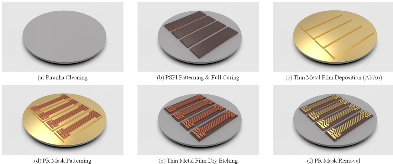
Figure 8. Thin-film metal test pattern fabrication process. (a) Piranha cleaning for removing organic residues from Si substrates, (b) Spin-coating, UV exposure, developing process, and Full curing in vacuum condition for PSPI patterning, (c) Thin metal film (Al and Au) deposition using an E-beam evaporation process. (d) Positive photoresist patterning for thin metal film etching mask, (e) The ICP-RIE-based dry etching process for thin metal film patterning, (f) The Oxygen plasma-based dry etching process for photoresist removing.
