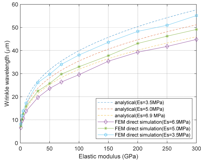
Figure 5. Wrinkling wavelength vs. elastic modulus of thin film as a function of substrate elasticity.
