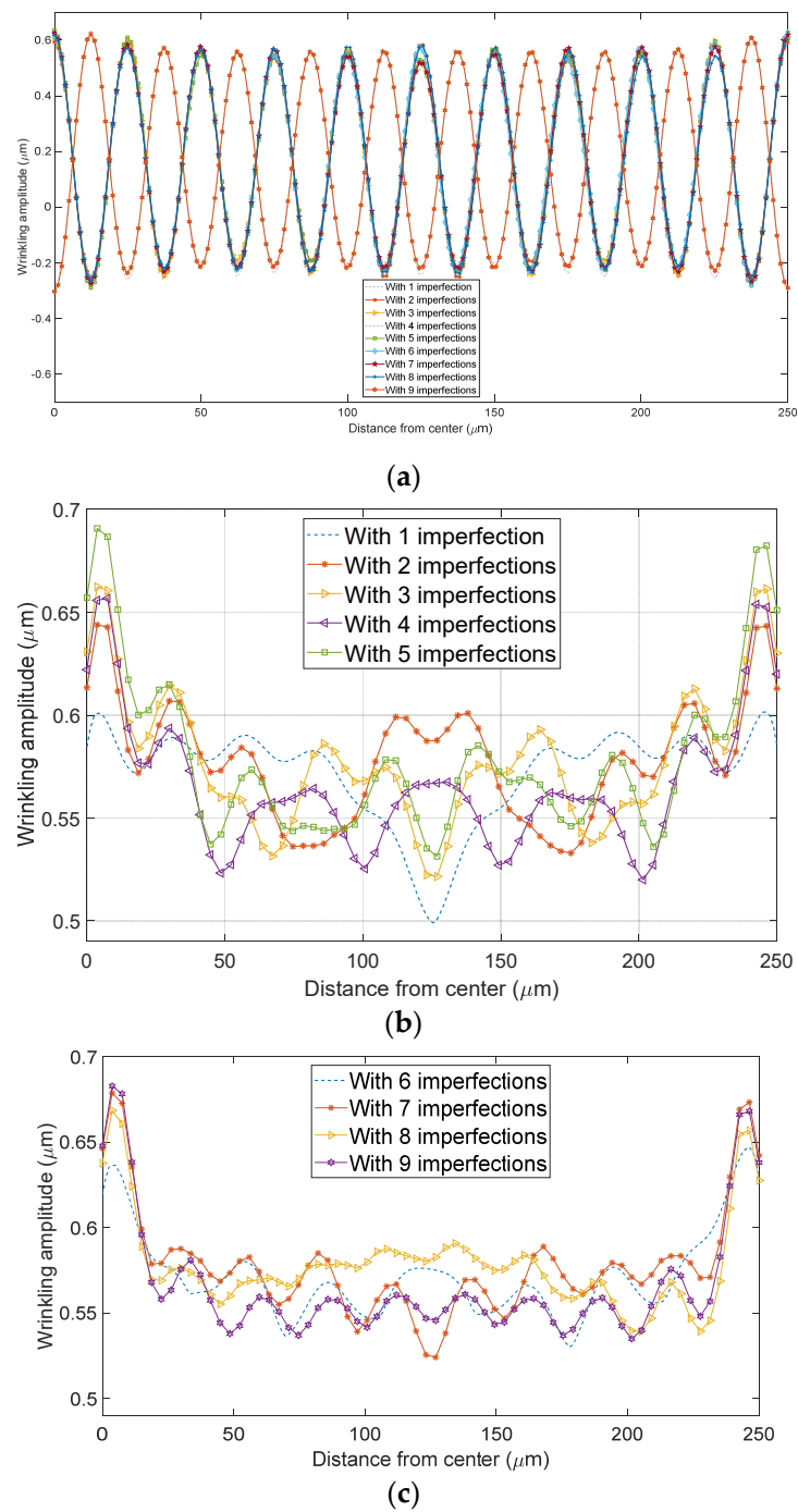
Figure 4. Wrinkling pattern as function of the number of imperfections. (a) Sinusoidal wrinkling pattern; (b) Envelope of the wrinkling pattern 1; (c) Envelope of the wrinkling pattern 2.
