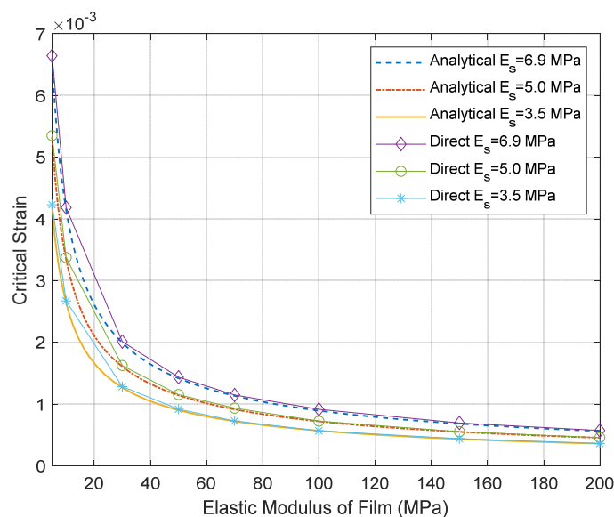
Figure 6. Critical strain as a function of elasticity of thin film for different substrate elasticity.
