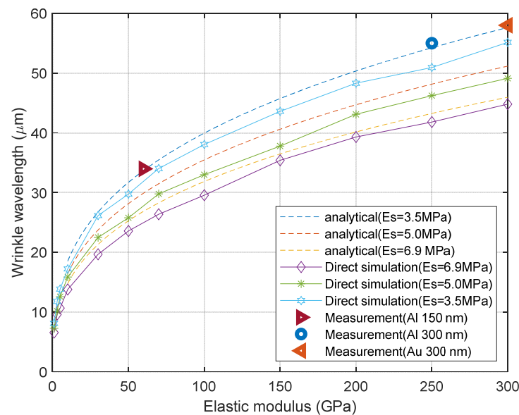
Figure 12. Elastic modulus extracted from wrinkling wavelength.
