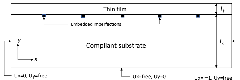
Figure 1. The 2D wrinkling model and boundary conditions.
