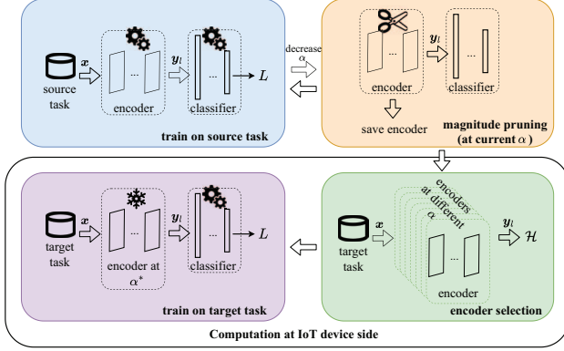
Figure 2. Schematic representation of the proposed ENTROPI algorithm. This approach trains a neural network in the source task in synergy with iterative magnitude pruning (with decreasing values of \alpha ). An encoder selection chooses the pruned model with the highest entropy, and finally, the pruned model is fine-tuned in the target task.
