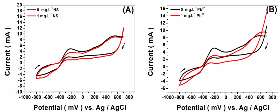
Figure 4. Cyclic voltammetry at 10 \text{ mV s}^{-1} of MFC anodic biofilm reached maturity after 11 days of MFC operation without and with 1 \text{ mg L}^{-1} of (A) NS antibiotic and (B) \text{Pb}^{2+} ions. Scan rate 10 \text{ mV s}^{-1} .
