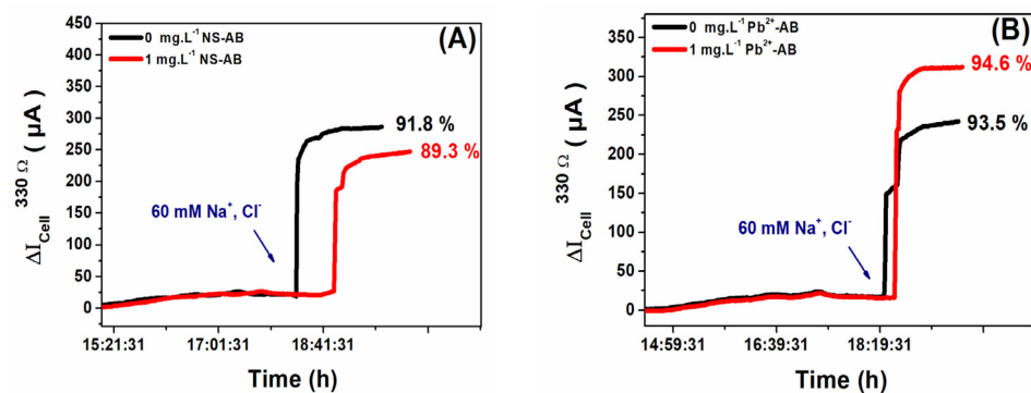
Figure 5. Effect of 60 \text{ mM } (\text{Na}^+, \text{Cl}^-) , \sigma \approx 7 \text{ mS cm}^{-2} , on output currents of biofilm-based MFCs non-adapted and adapted to different toxicity concentrations: (A) NS antibiotic and (B) \text{Pb}^{2+} ions. These experiments were performed after the maturation/adaptation process of biofilms in a fresh medium with 10 \text{ mM NaAc} substrate. The anode and cathode were connected across a 330 \Omega external resistor.
