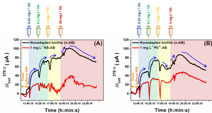
Figure 6. Change in output currents of mature electroactive biofilm-based MFCs non-adapted (black line) and adapted (red line) to 1 \text{ mg L}^{-1} of NS or \text{Pb}^{2+} ions in fresh buffered wastewater with only 60 mM ( \text{Na}^+ , \text{Cl}^- ), \sigma \approx 7 \text{ mS cm}^{-2} , and 10 mM NaAc. Biofilms were challenged with successive additions of (A) NS in the concentration range 0.01–20 \text{mg L}^{-1} and (B) \text{Pb}^{2+} in the concentration range 0.01–5 \text{mg L}^{-1} .
