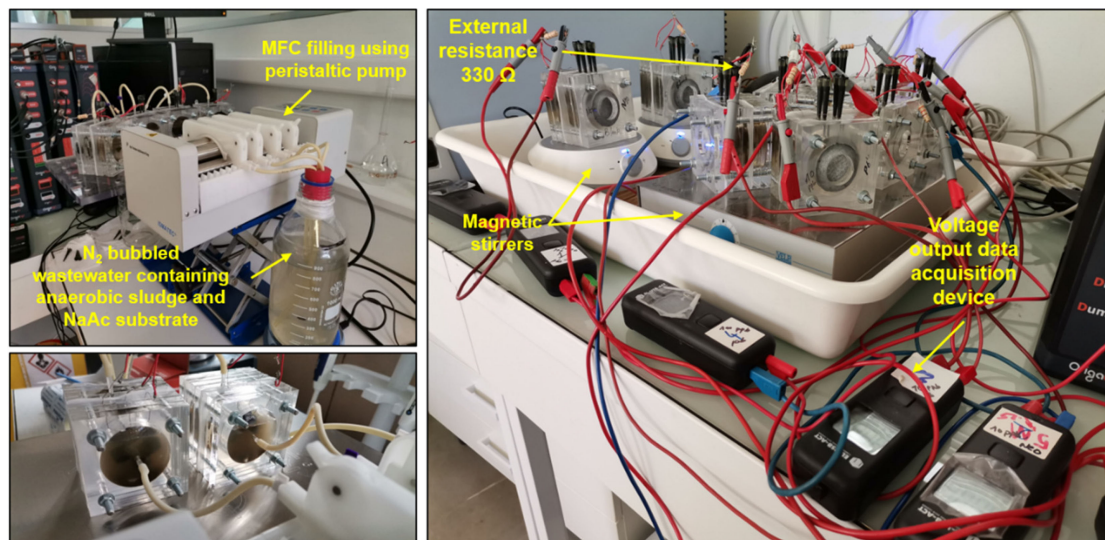
Figure 2. Pictures illustrating MFC filling with degassed wastewater containing anaerobic sludge and NaAc as carbon source using peristaltic pumping. MFC reactors, at the start point of experimentation, were subjected to different concentrations of pollutants ( \text{Pb}^{2+} ions and NS) for biofilm growth/adaptation to pollutants.
