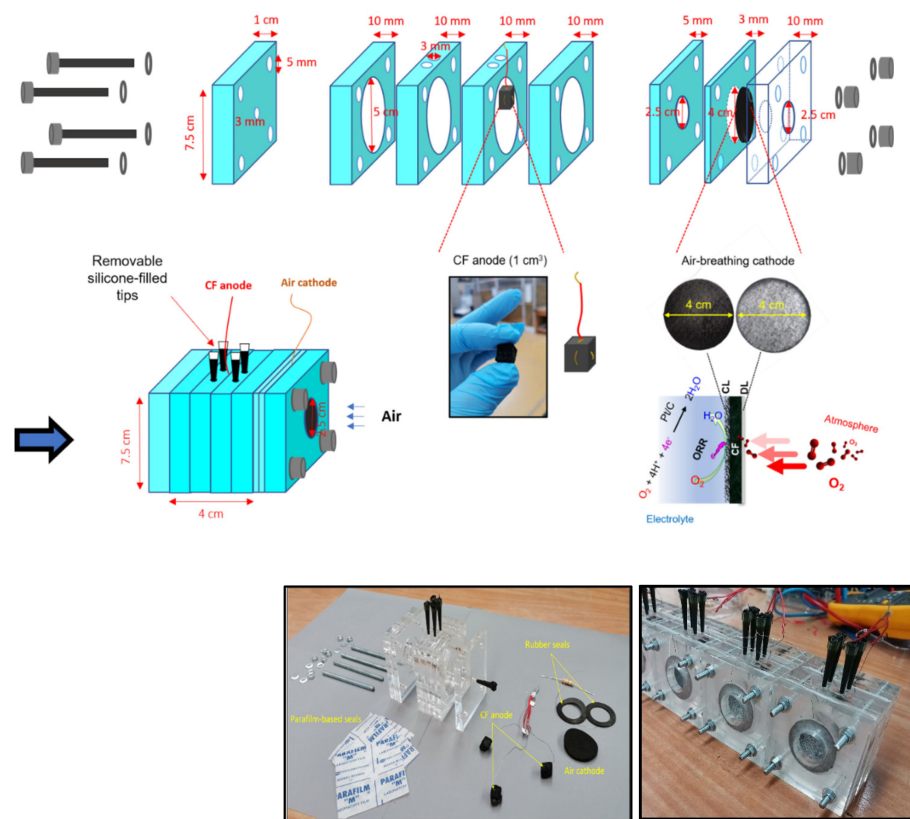
Figure 1. Schematic illustration of the components used for MFC biosensor construction and photos of pieces used in the final MFC biosensor assembly (left) and final forms of air-cathode, single-chamber MFC biosensors equipped with CF anodes and air cathodes after assembling (right).
