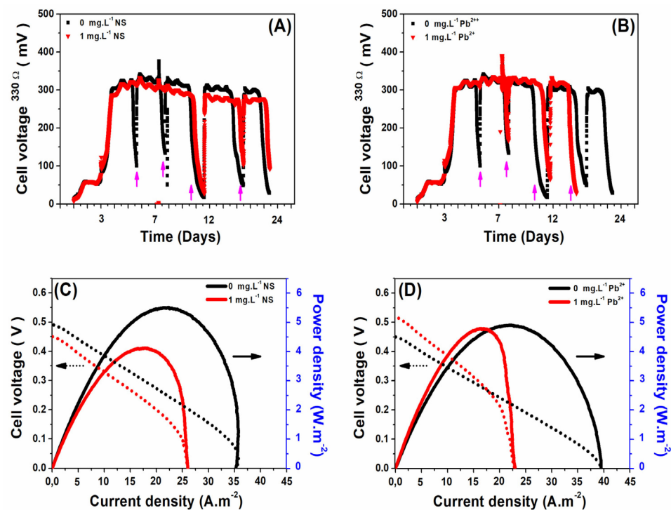
Figure 3. Voltage outputs produced during biofilm growth on CF anodes in MFCs operating separately without and with 1 \text{ mg L}^{-1} of (A) NS antibiotic and (B) \text{Pb}^{2+} ions. The pink arrows represent the injection of 10 mM NaAc into the medium. Polarization and power density curves of non-adapted and adapted biofilm-based MFCs at different concentrations of (C) NS antibiotic or (D) \text{Pb}^{2+} ions were recorded using LSV. The biofilm on the CF anode in all MFC reactors reached maturity after 11 days of MFC operation. Scan rate, 10 \text{ mV s}^{-1} .
