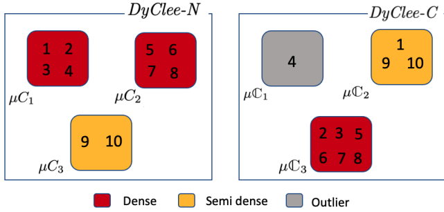
Fig. 3. The outlier problem
