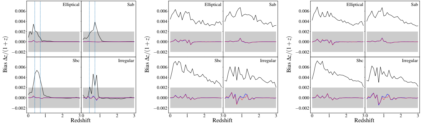
Fig. 7. Bias in the photometric redshifts due to passband variations as a function of redshift in the MegaCam ugriz + Euclid Y_E J_E H_E configuration. Each plot shows the bias for the four CWW templates, as indicated. Left : only the r passband is variable; centre : all passbands are variable; right : all passbands are variable, and four exposures have been stacked. In the left plot, the vertical dashed lines indicate the redshifts where the Balmer break enters and exits the r passband. The different curves show the bias when the passband variations are ignored (black line), or when the full central passbands corrected for the shifts in mean wavelengths (blue line) are used. The dashed red lines show the bias when the second-order polynomial correction on the flux presented in Sect. 5.2 is used. We point out that the blue and red lines are very close, so that the blue line is often barely visible.
