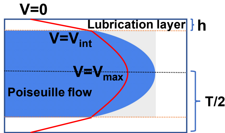
Figure 2. Velocity profile inside the slit with a lubrication layer between the droplet and the slit walls. The flow is a 2D Poiseuille flow inside the blue region.
