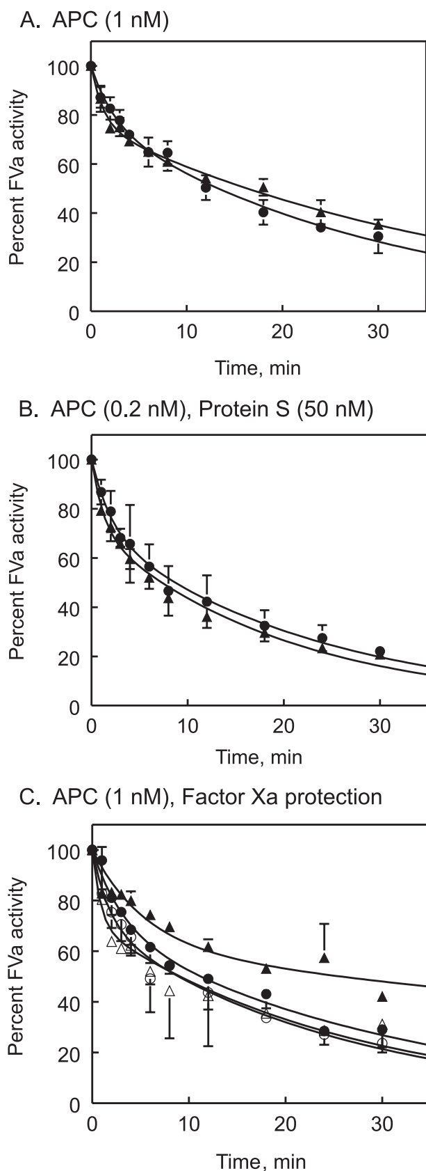
FIGURE 5. 499-505 VIII FVa is inactivated by APC essentially the same as wild type FVa. A , inactivation of FVa variants over time by 1 nM APC alone as described under "Materials and Methods." ▲ = wild type FVa; ● = 499-505 VIII FVa. B , inactivation of FVa variants over time by 0.2 nM APC and 50 nM protein S as described under "Materials and Methods." ▲ = wild type FVa; ● = 499-505 VIII FVa.
