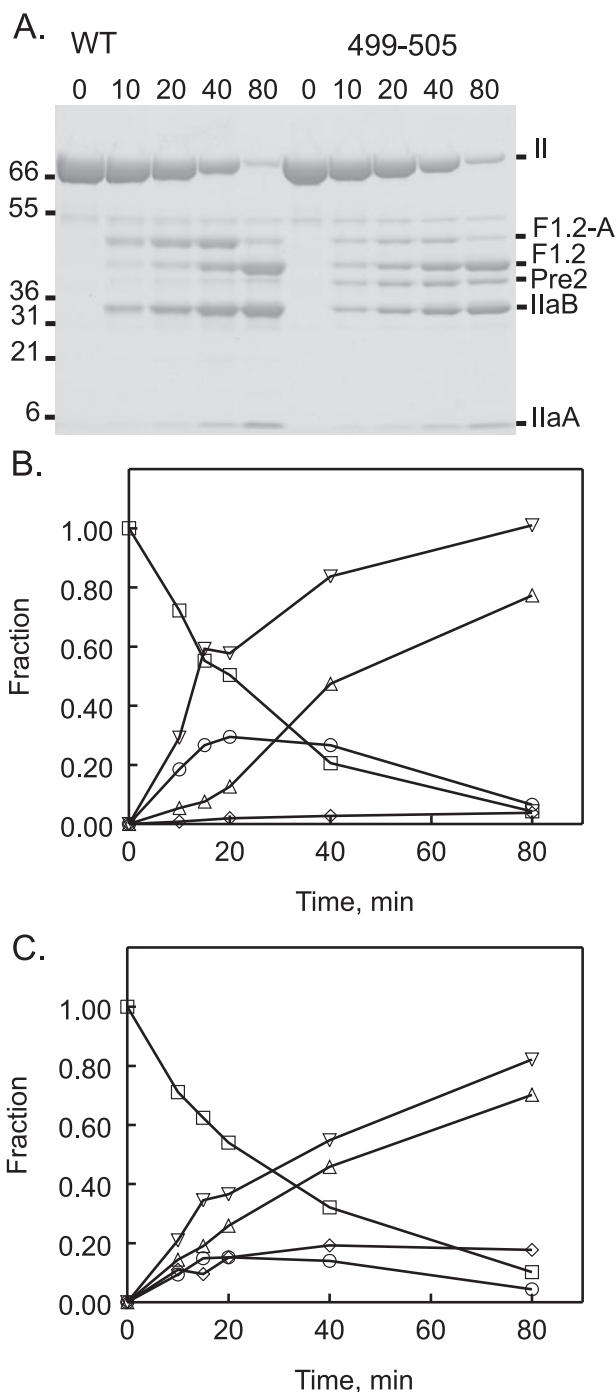
FIGURE 4. Cleavage of prothrombin by the prothrombinase complex containing wild type FVa or 499–505 VIII FVa. A, reduced Coomassie Blue-stained gel of a time course, in minutes, of prothrombin cleavage. The cleavage reactions are described under "Materials and Methods." Samples were reduced with dithiothreitol, alkylated with iodoacetamide, and run on a 4–12% BisTris gel with MOPS-SDS buffer from Invitrogen. Molecular weight standards are indicated on the left, and prothrombin fragment identifications are indicated on the right. II = intact prothrombin; F1.2-A = amino acids 1–320; F1.2 = amino acids 1–271; Pre2 = amino acids 272–579; IIaB = amino acids 321–579; and IIaA = amino acids 272–320. B and C, quantitative densitometry of wild type FVa (B) and 499–505 VIII FVa (C) from the gel in panel A. The y axis is the fraction of the maximum possible fragment concentration. □ = II; ○ = F1.2-A; △ = F1.2; ◇ = Pre2; and ▽ = IIaB. Results are combined from 2 different experiments.
