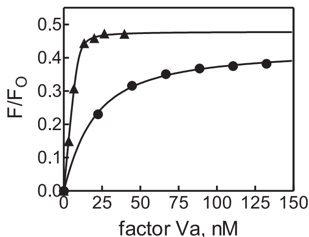
FIGURE 3. 499–505 VIII FVa binds with greatly reduced affinity to FI-FXa. FVa was titrated into FI-FXa i , and fluorescence intensity change was monitored. \blacktriangle = wild type FVa; \bullet = 499–505 VIII FVa. Data were fit to a quadratic equation from which the K_d was derived. Standard deviations were too small to be visible on this graph.
