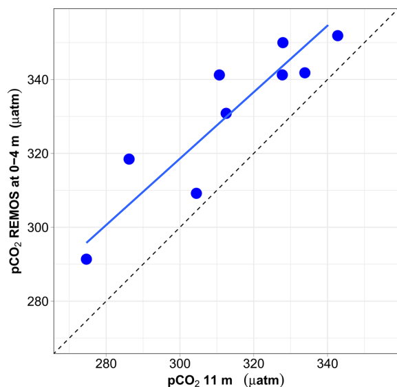
Figure 10. Relationship between surface p\text{CO}_2 (0–4 m) (estimated from pH and salinity-derived A_T ) and p\text{CO}_2 at 11 m. Both values are expressed at in situ temperature. The mean and median difference between the two p\text{CO}_2 values are about 17 \mu\text{atm} . The major-axis regression line is shown in blue, whereas the 1 : 1 relationship is depicted by a dotted black line.
