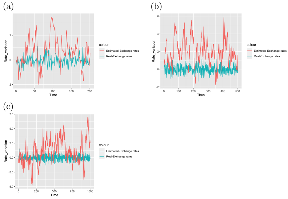
FIGURE 9. Comparison between exchange rates prediction with Stable driven OUP with sample size n = 200 (a); sample size n = 500 (b) and sample size n = 1000 (c).
