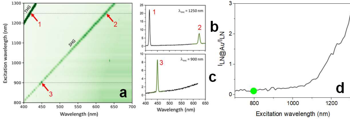
Figure 5. (a) Image of the emission spectra (x axis) as a function of the laser wavelength (y axis, 10-nm wavelength increments) for the LN@Au NPs suspension. Specific spectra at (b) 1250 nm excitation and (c) 900 nm excitation extracted from (a) showing SHG peaks at 625 nm (peak 2) and 450 nm (peak 3), respectively. Note that Third Harmonic Generation is also detected for laser wavelengths above 1200 nm (peak 1). (d) Normalized ratio of the SHS signal from LN@Au and LN suspensions as a function of the excitation wavelength. Normalization of the spectral response was made at \lambda = 800 nm according to the procedure described in the text (green circle).
