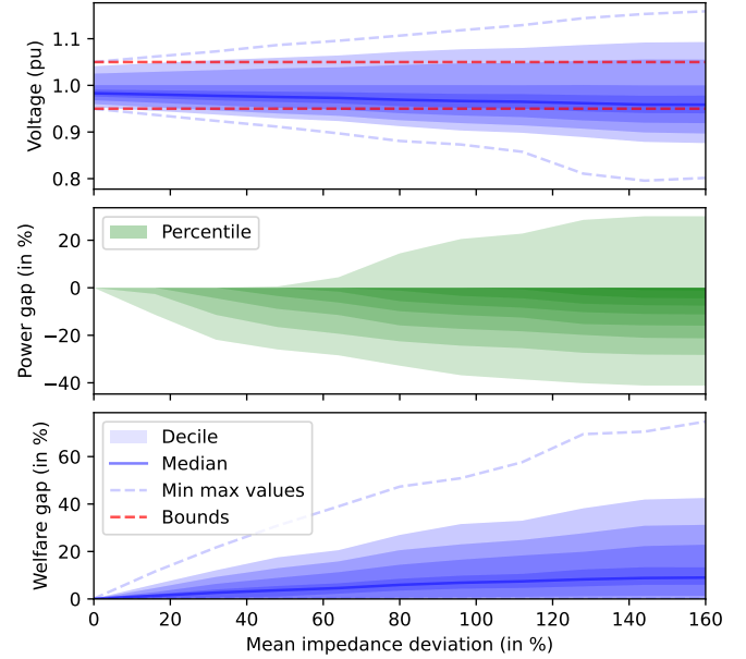
Fig. 3. Sensitivity of AC-OPF-SOC results depending on the average of impedance estimation errors. Top: repartition of voltages at each bus; middle: repartition of power injection deviation; bottom: suboptimality of social welfare. Permissible limits in red, deciles and percentiles in colored areas, extreme values observed in dotted blue line. Results observed on ELVF under a truncated normal distribution.
