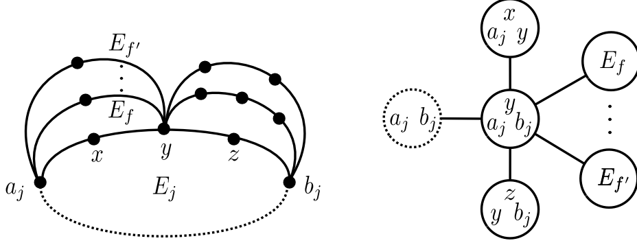
Figure 14: Graph (left) and tree-decomposition (right) of G_{i+1} with \ell_j = 4 and Att(E_j) \subseteq \{a_j, y, b_j\} .
