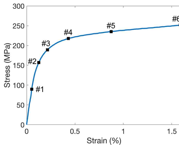
Fig. 5 Macroscopic nominal stress-strain curve. The squares overlaid on the curve mark the instances at which quantities are reported in the rest of the paper
