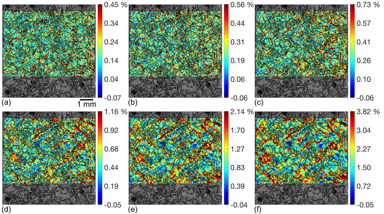
Fig. 6 Von Mises in-plane strain fields at the instances a) #1, b) #2, c) #3, d) #4, e) #5 and f) #6 (marked in Fig. 5 ) projected onto a map of the initial microstructure of the sample with overlaid grain boundaries
