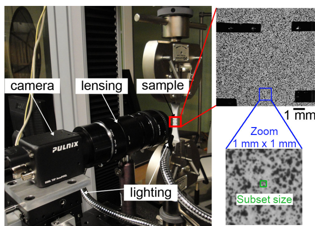
Fig. 2 Experimental setup for in-situ in-plane strain field measurements under uniaxial loading. The inset shows the area of the sample imaged by the camera as well as the speckle pattern
