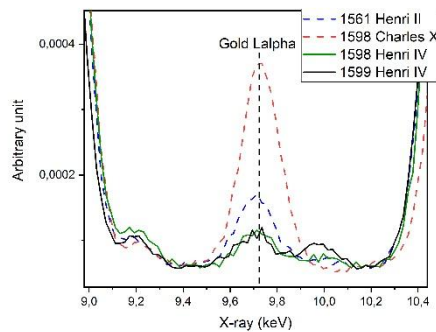
Figure 9 XRF spectra - gold La lines of silver coins
