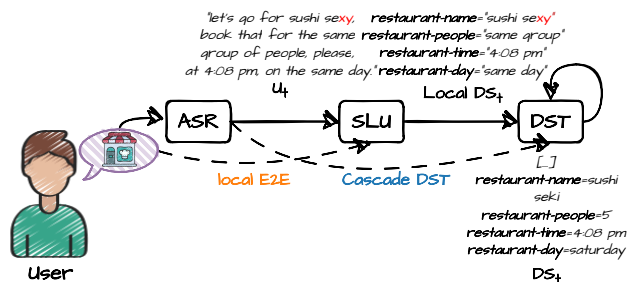
Fig. 1. Spoken Dialogue State Tracking alternatives. Red characters indicate potential cascading errors.
