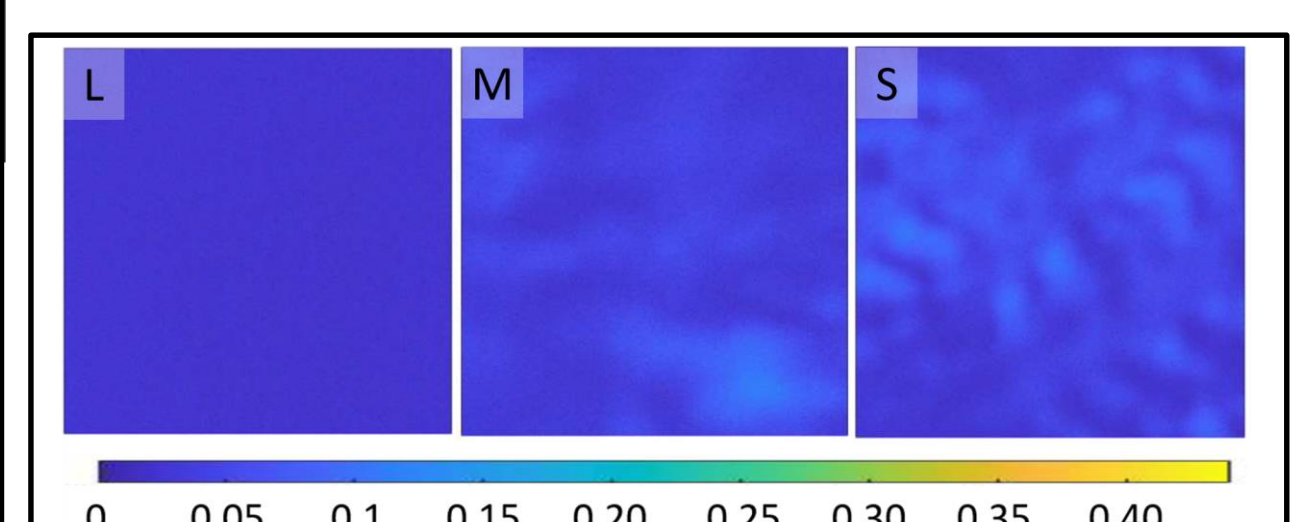
Fig. 6. Fake DoLP examples for sky drift level estimation. L : low sky drift, M : medium, S : strong sky drift.
