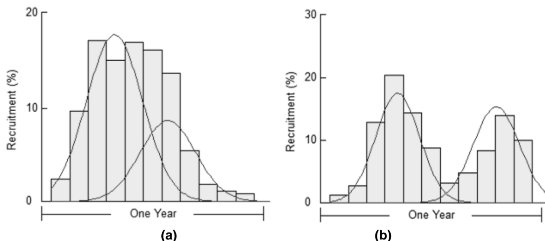
Fig. 4. Illustration of recruitment curves and their peaks in chez S. tanganyicae at at Nyamugari (a) and Kajaga (b) beaches
