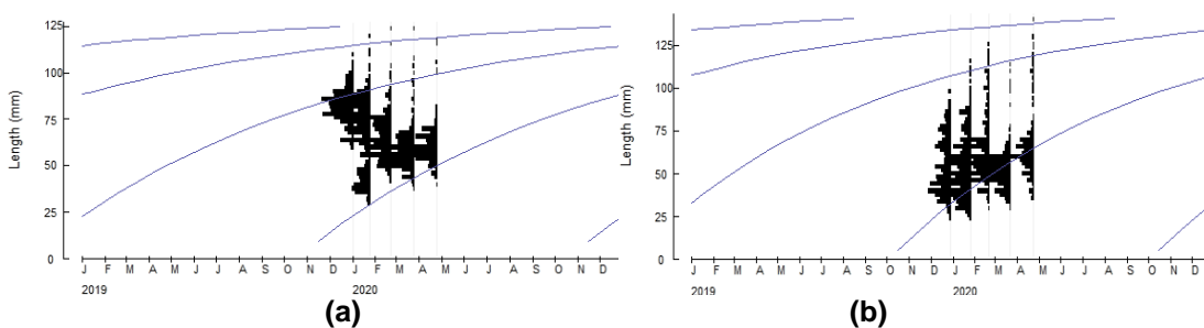
Fig. 3. Von Bertalanffy growth curves for L. miodon : (a) Nyamugari Beach and (b) Kajaga Beach
