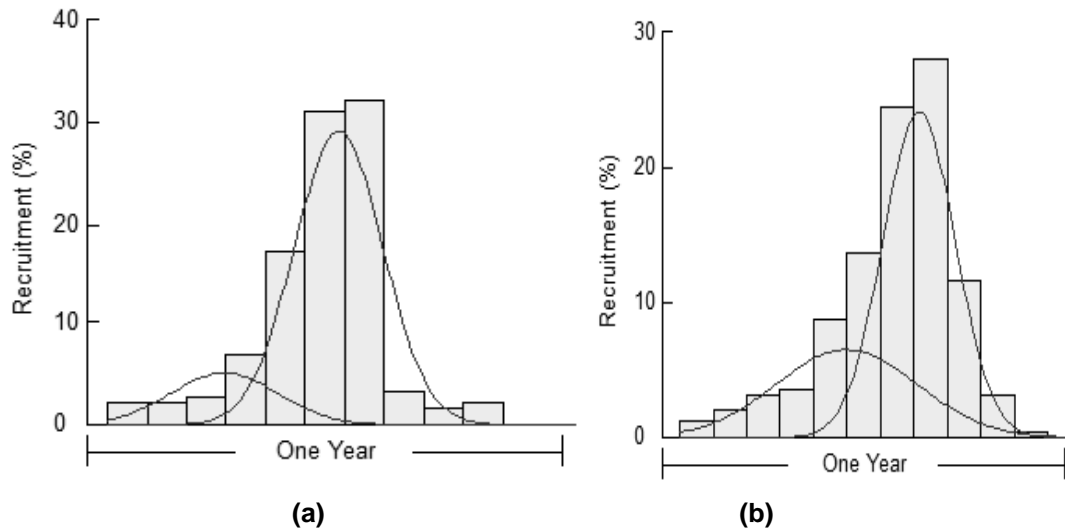
Fig. 5. Illustration of recruitment curves and their peaks in L. miodon at at Nyamugari (a) and Kajaga (b) beaches
