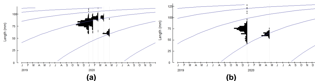
Fig. 2. Von Bertalanffy growth curves for S. tanganicae : (a) Nyamugari Beach and (b) Kajaga Beach
