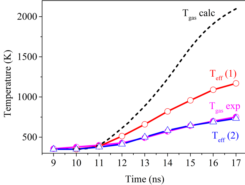
Figure 13. Comparison of calculated non-convoluted T_{\text{gas}} \text{ (calc)} , calculated convoluted over the region of measurements ( T_{\text{eff}} \text{ (1,2)} - see text for the details) and the experimentally measured T_{\text{gas}} \text{ (exp)} (Figure 67 of [20]) gas temperatures at the probe point r = 0 , z = 0.5 mm.
