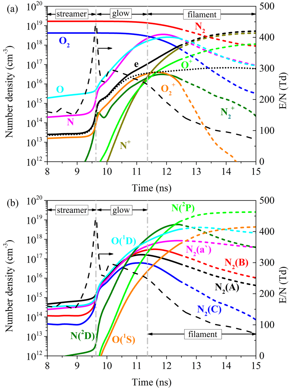
Figure 10. Kinetic curves of selected (a) ground and charged, and (b) excited species close to the cathode ( r = 0, z = 0.05 mm). The bold solid curves refer to times when n_e \leq 10^{18} cm -3 , and short dashed curves indicate when n_e \geq 10^{18} cm -3 . The dotted black line in (a) is the electron density without consideration of reactions (13), (14), and (15) (shown below). The reduced electric field strength is plotted as a reference.
