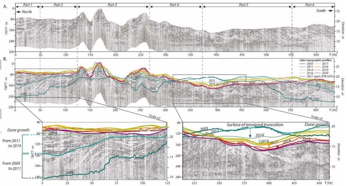
FIGURE 8. (a) Processed versions of the profile LS-1 acquired with 500 MHz frequency antennae. GPR data are given in nanosecond (ns) two-way travel time (TWTT) and elevations are with reference to mean sea-level (amsl). (b) Topographic survey drawn on (a). Localization of LS-1 is indicated.
