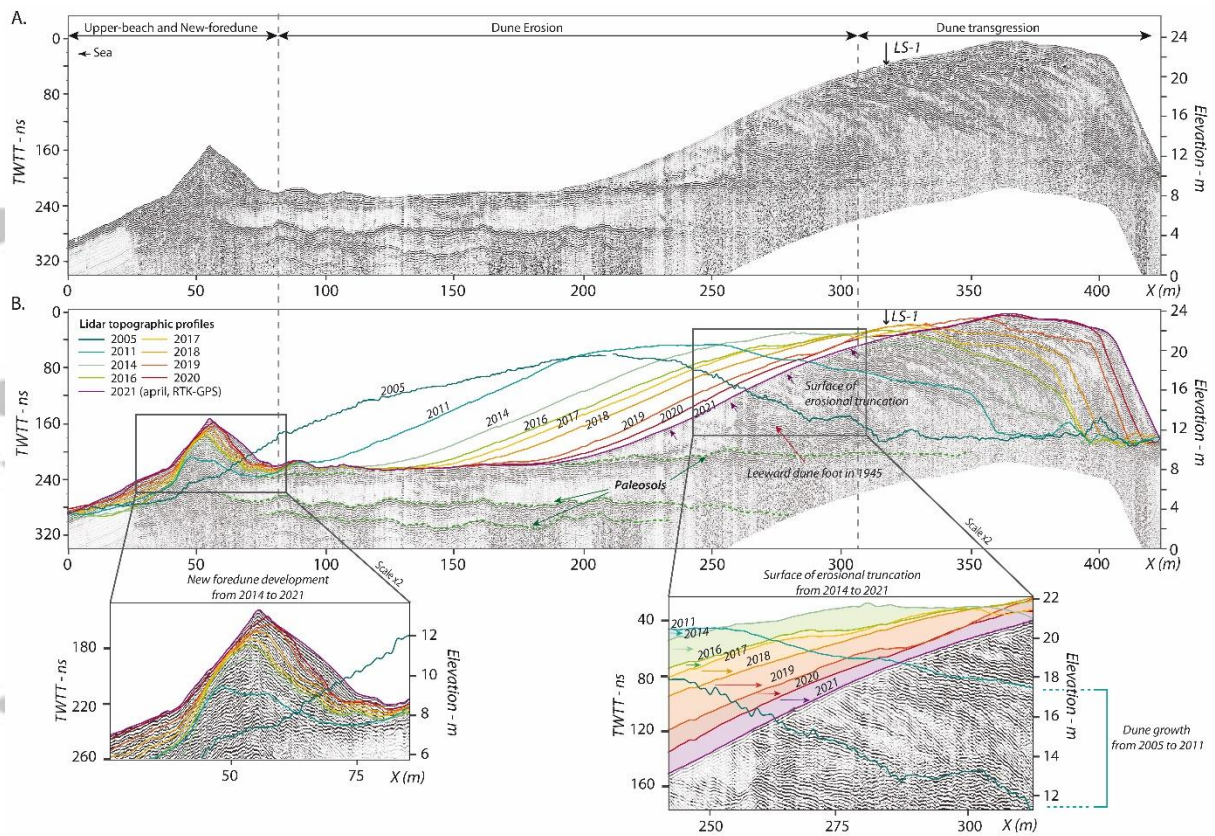
FIGURE 7. (a) Processed versions of the profile CS-3 acquired with 500 MHz frequency antennae. GPR data are given in nanosecond (ns) two-way travel time (TWTT) and elevations are with reference to mean sea-level (amsl). (b) Topographic survey drawn on (a). Localization of LS-1 is indicated and also the leeward dune foot position in 1945.
