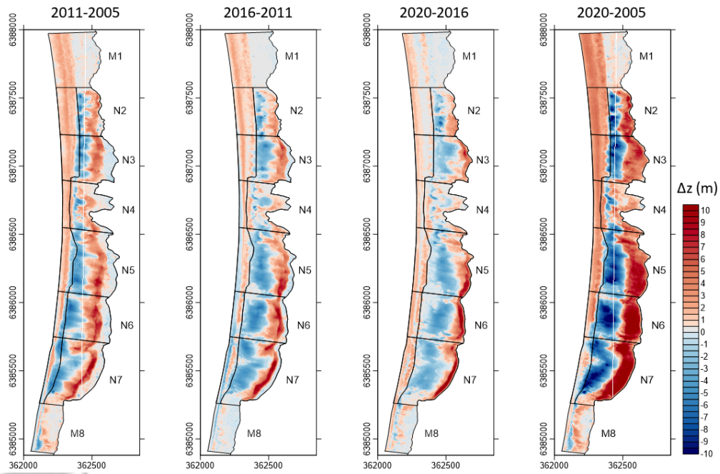
FIGURE 9. DTM difference plot of the Trencat dune during different periods of Stage III. Black lines correspond to the limits of the foredune, transgressive dune and landward dune, and of each area.
