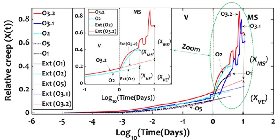
Fig. 15 Separating viscoelastic and mechanosorptive behaviour in the case of Okoume. X_{VE} : viscoelastic contribution obtained by linear extrapolation of 1-day creep; X_{MS} mechanosorptive contribution obtained by difference at the end of the test
