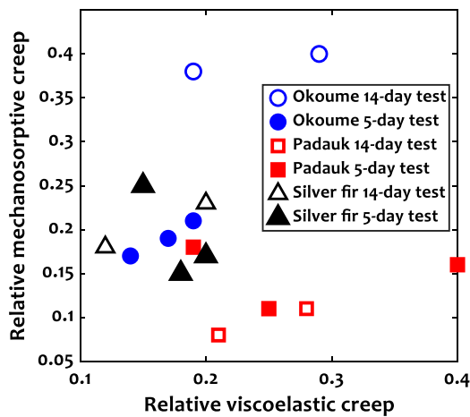
Fig. 16 Relationship between the contribution to relative creep of mechanosorption and viscoelasticity: empty symbols, 14-day tests; filled symbols: 5-day test
