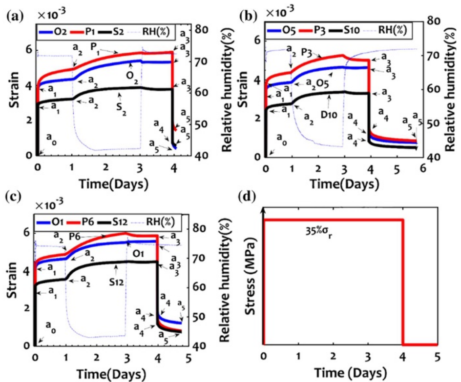
Fig. 10 Creep at 35% stress level for 4 days followed by 0–2 days of recovery; a test 1, Okoume (O2), Padauk (P1) and Silver fir (S2); b test 2, Okoume (O5), Padauk (P3) and Silver fir (S10); c test 3, Okoume (O1), Padauk (P6) and Silver fir (S12); d applied stress
