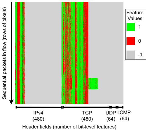
Figure 2: Color processed synthetic data for Amazon: all packets (rows of pixels) are of the protocol type TCP. -1 denotes vacant header fields.
