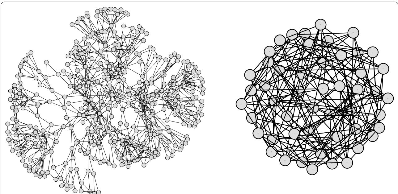
Fig. 2 Tamaki’s tree-decomposer [23] has a harder time with the right, more tangled instance (50 nodes, 175 edges, treewidth 25 computed in 79s) than with the larger instance on the left (465 nodes, 1004 edges, treewidth 9 computed in 0.5s), illustrating that tangledness is a more important factor than size. Indeed, both instances display a tangledness that already exceeds what we expect to see in real-world phylogenetic networks. The instances are ex065 (right) and ex011 (left) of the PACE2017 challenge [22]
