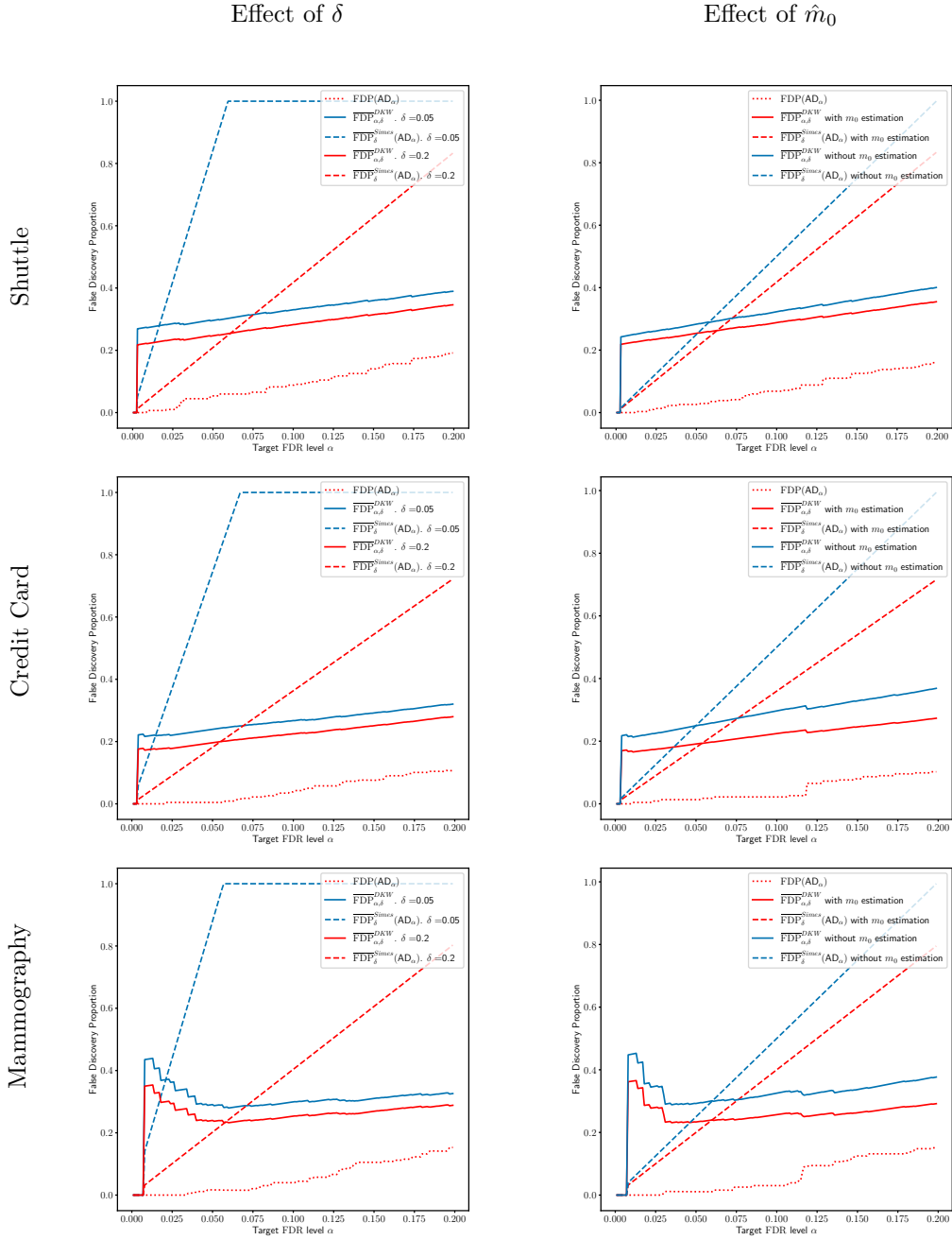
Figure 7: Same curves as Figure 6 (left), but only for two-class classification (adaptive, red). Left: for comparison, the bounds \overline{\text{FDP}} were also plotted for a smaller \delta = 0.05 value (blue). Right: for comparison, bounds \overline{\text{FDP}} also plotted without an estimator of m_0 (taking m instead of \hat{m}_0 ).
