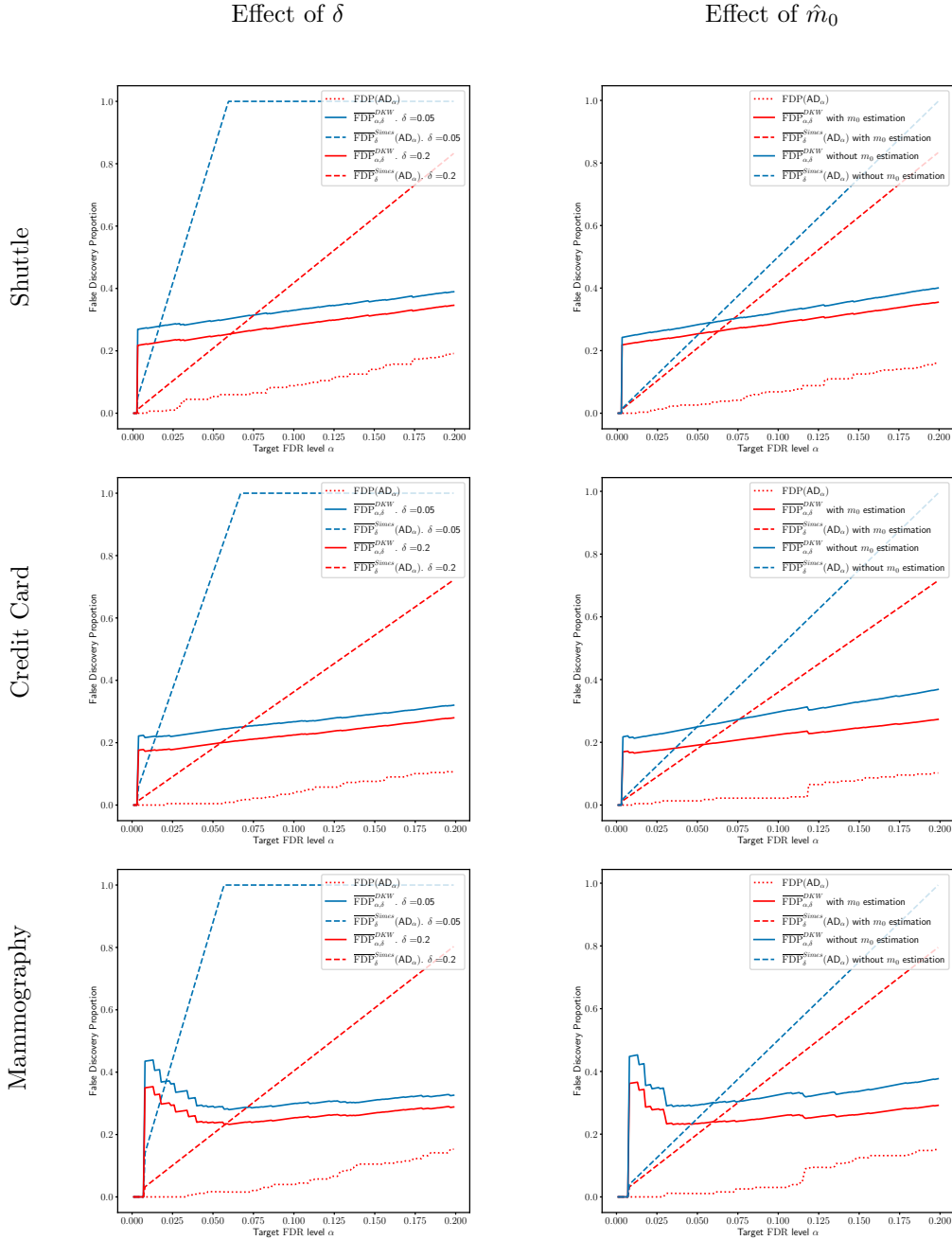
Figure 7: Same curves as Figure 6 (left), but only for two-class classification (adaptive, red). Left: for comparison, the bounds \overline{FDP} were also plotted for a smaller \delta = 0.05 value (blue). Right: for comparison, bounds \overline{FDP} also plotted without an estimator of m_0 (taking m instead of \hat{m}_0 ).
