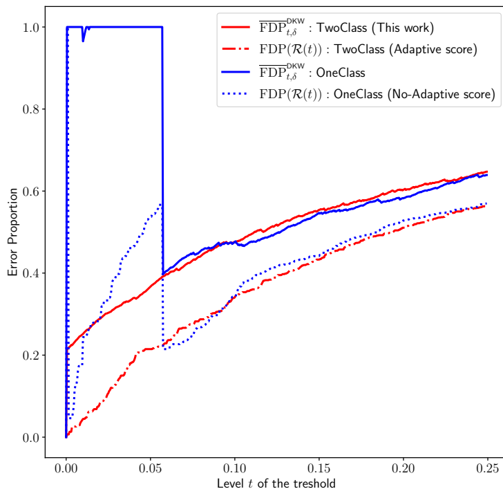
Figure 3: Plot of FDP(\mathcal{R}(t)) (22)(23) (dashed) and bound \overline{FDF}_{t,\delta}^{DKW} (24) (solid, \delta = 0.2 ) in function of the threshold t for \mathcal{R}(t) (23) with a score obtained either with a one-class classification (non-adaptive) or a two-class classification (adaptive).
