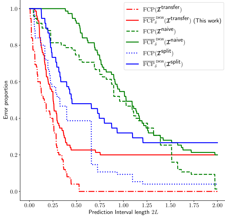
Figure 2: Plot of \text{FCP}(\mathcal{Z}) (15) (dashed) and bound \overline{\text{FCP}}_{\hat{\alpha}(L),\delta}^{\text{DKW}} (21) (18) (solid, \delta = 0.2 ) in function of interval length 2L in the same setting and procedures as in Figure 1.
