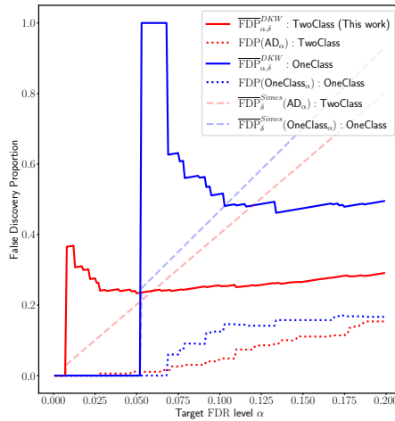
Figure 6: Left: \overline{\text{FDP}}(\text{AD}_\alpha) (22)(48) (dotted) and bounds \overline{\text{FDP}}_{\alpha,\delta}^{\text{DKW}} (50) (solid) \overline{\text{FDP}}_{\alpha,\delta}^{\text{Simes}} (51) (dashed) ( \delta = 0.2 ) in function of the nominal FDR-level \alpha . Right: corresponding TDP (52). In AdaDetect, the score is obtained either with a one-class classification (non-adaptive, blue) or a two-class classification (adaptive, red); higher is better.
