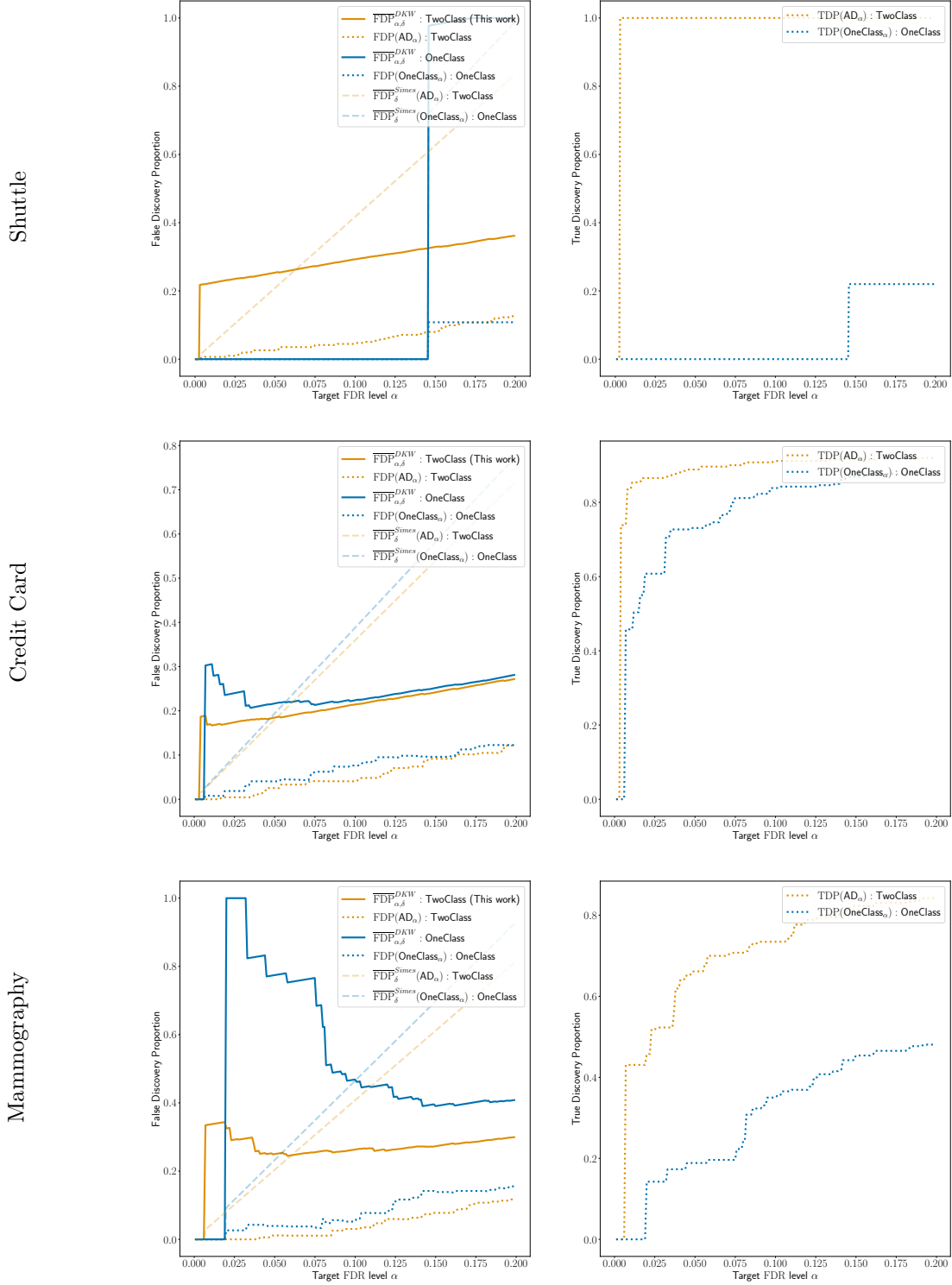
Figure 7: Left: \overline{\text{FDP}}(\text{AD}_{\alpha}) (22)(49) (dotted) and bounds \overline{\text{FDP}}_{\alpha, \delta}^{\text{DKW}} (51) (solid) \overline{\text{FDP}}_{\alpha, \delta}^{\text{Simes}} (52) (dashed) ( \delta = 0.2 ) in function of the nominal FDR-level \alpha . Right: corresponding TDP (53). In AdaDetect, the score is obtained either with a one-class classification (non-adaptive, blue) or a two-class classification (adaptive, orange); higher is better.
